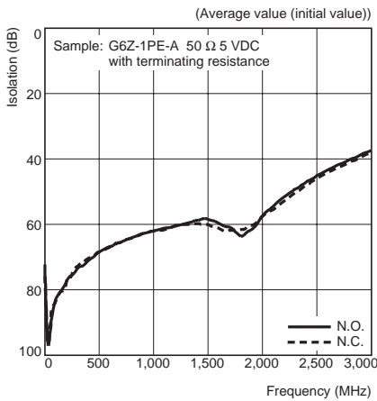
High-frequency Characteristics at 50 Ω (Isolation)
