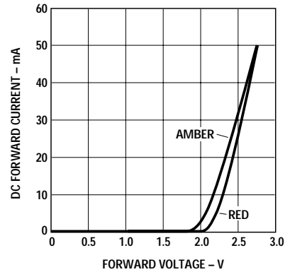
Figure 2a. Forward Current vs. Forward Voltage for Option -xxRxx, -xxSxx, -xxTxx, -xxUxx, -xxVxx and -xxYxx.
