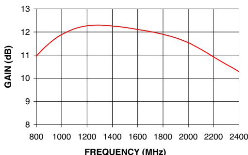
ZX60-2411BM+ GAIN
