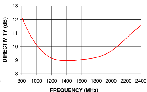
ZX60-2411BM+ DIRECTIVITY
