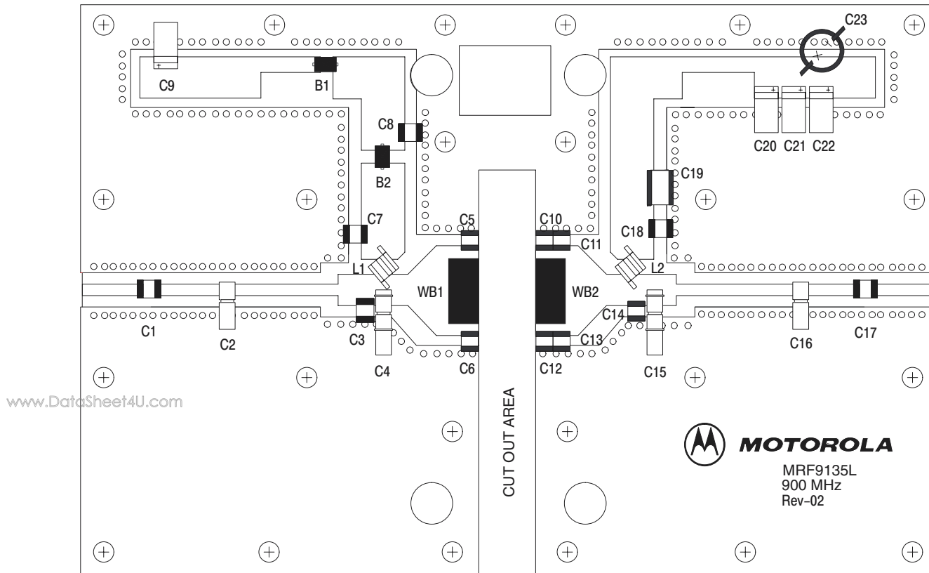
Figure 2. 880 MHz Test Circuit Component Layout
