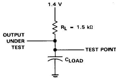
FIGURE 2. STANDARD TEST LOAD CIRCUIT
