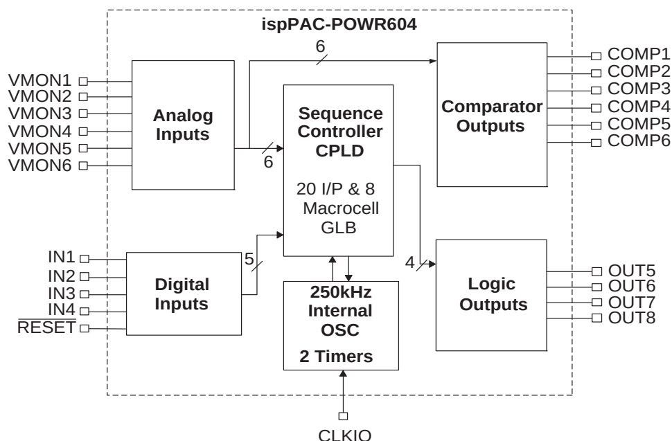
Figure 2-1. ispPAC-POWR604 Block Diagram
