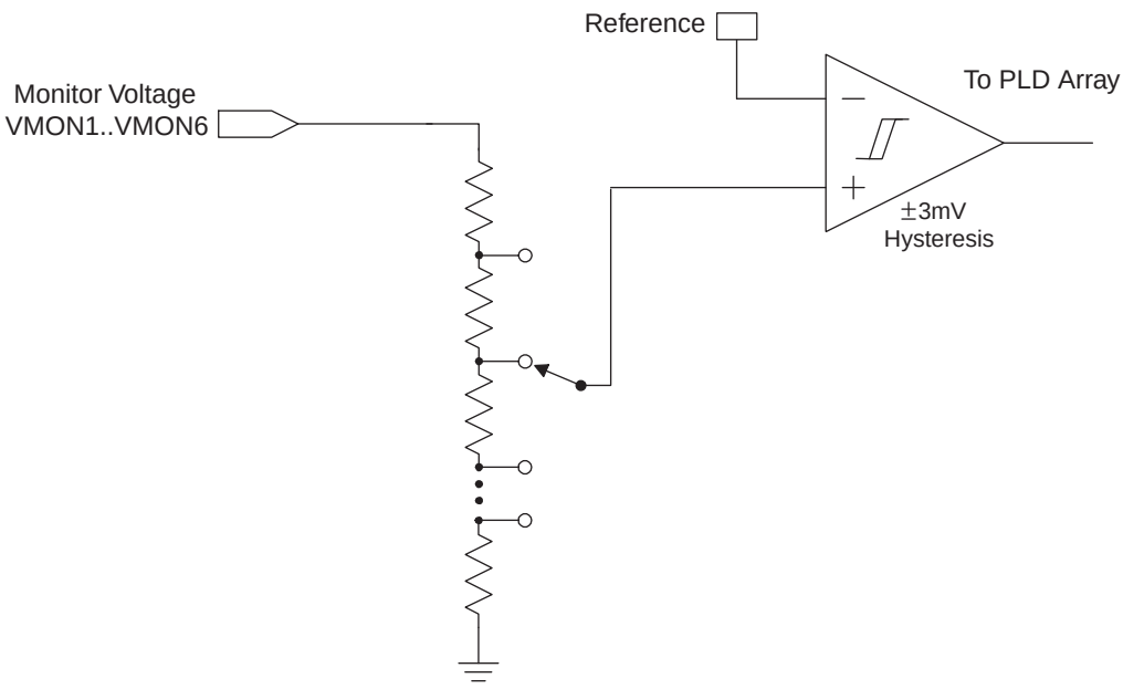
Figure 2-2. Voltage Monitors
