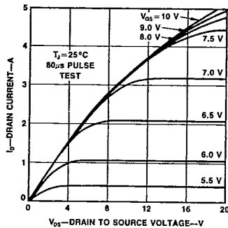
Figure 3 Output Characteristics
