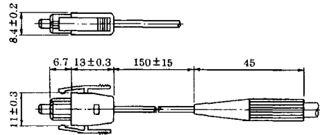
(1) Fiber optic connector
