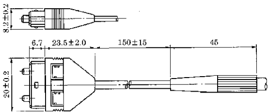
(2) Optical fiber
