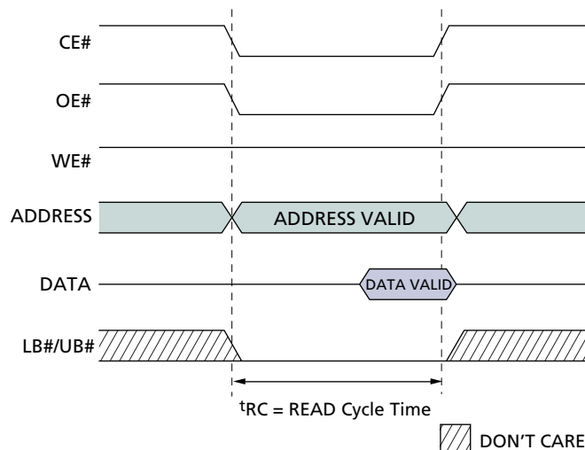
Figure 5: READ Operation
