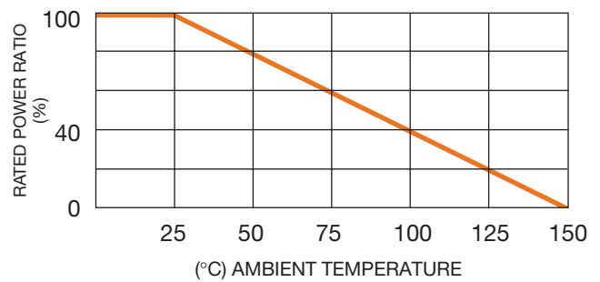
DERATING CURVE
