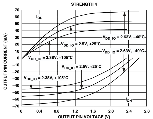
Figure 29. Typical Drive Currents at Strength 4
