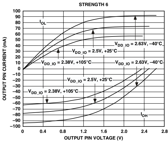
Figure 31. Typical Drive Currents at Strength 6
