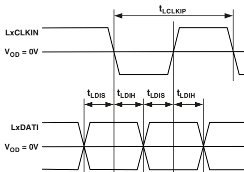
Figure 24. Link Ports—Data Input Setup and Hold 1
