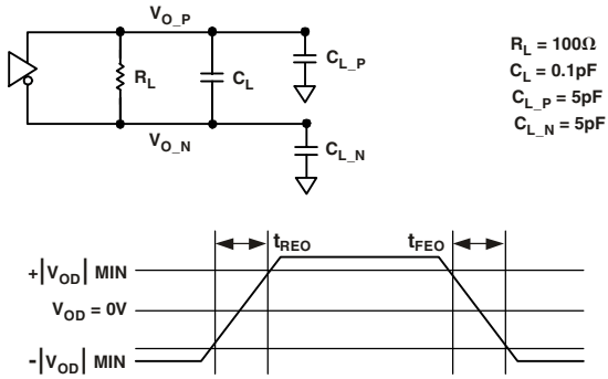
Figure 18. Link Ports—Differential Output Signals Transition Time
