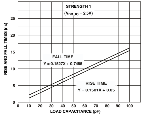
Figure 37. Typical Output Rise and Fall Time (10%–90%, V_{DD\_IO} = 2.5V ) vs. Load Capacitance at Strength 1
