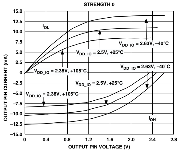
Figure 25. Typical Drive Currents at Strength 0
