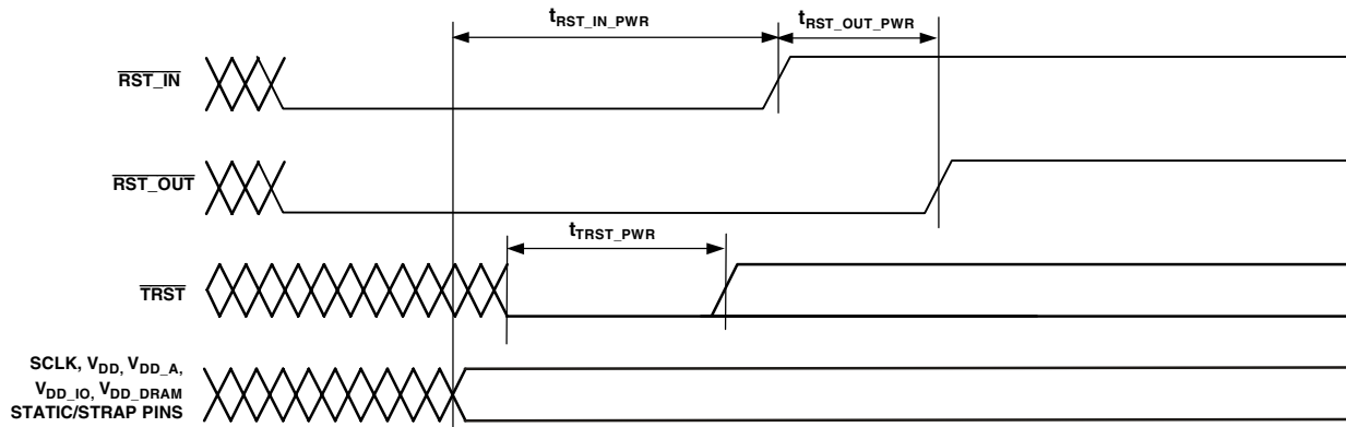
Figure 12. Power-Up Reset Timing
