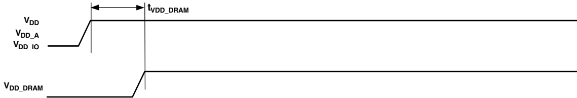
Figure 11. Power-Up Timing
