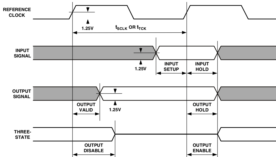
Figure 14. General AC Parameters Timing
