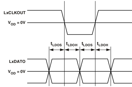
Figure 19. Link Ports—Data Output Setup and Hold 1
