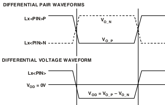
Figure 16. Link Ports—Signals Definition
