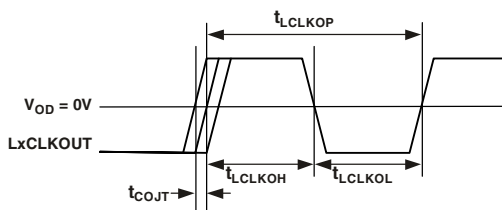
Figure 17. Link Ports—Output Clock
