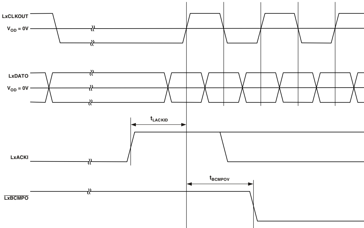
Figure 20. Link Ports—Transmission Start
