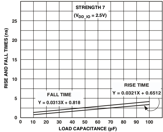
Figure 43. Typical Output Rise and Fall Time (10%–90%, V_{DD\_IO} = 2.5 V ) vs. Load Capacitance at Strength 7
