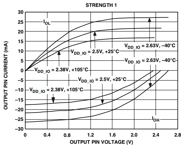
Figure 26. Typical Drive Currents at Strength 1
