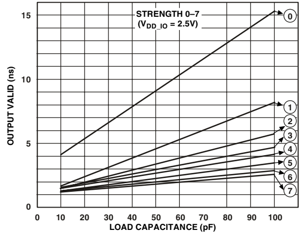
Figure 44. Typical Output Valid ( V_{DD\_IO} = 2.5 V ) vs. Load Capacitance at Max Case Temperature and Strength 0–7 1
