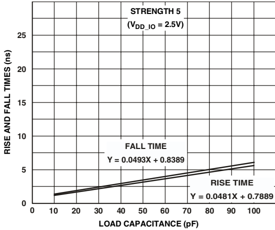
Figure 41. Typical Output Rise and Fall Time (10%–90%, V_{DD\_IO} = 2.5 V ) vs. Load Capacitance at Strength 5
