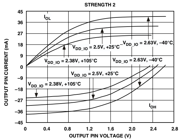
Figure 27. Typical Drive Currents at Strength 2
