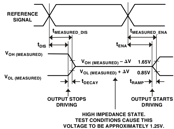
Figure 34. Output Enable/Disable
