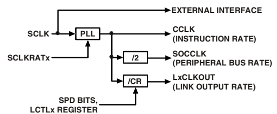
Figure 5. Clock Domains
