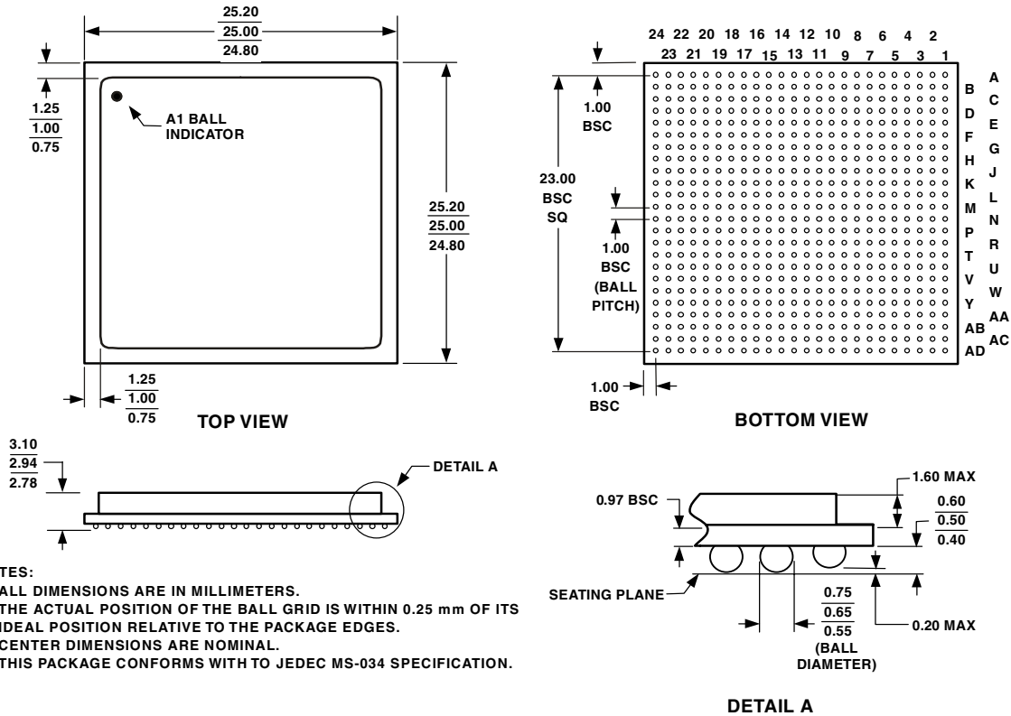
Figure 46. 576-Ball BGA_ED (BP-576)
