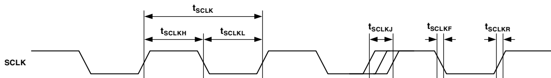
Figure 9. Reference Clocks—System Clock (SCLK) Cycle Time
