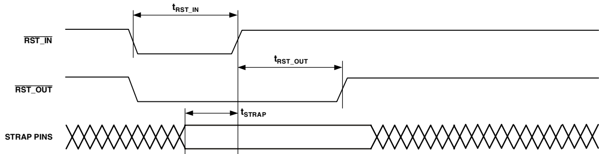
Figure 13. Normal Reset Timing
