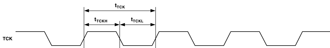
Figure 10. Reference Clocks—JTAG Test Clock (TCK) Cycle Time
