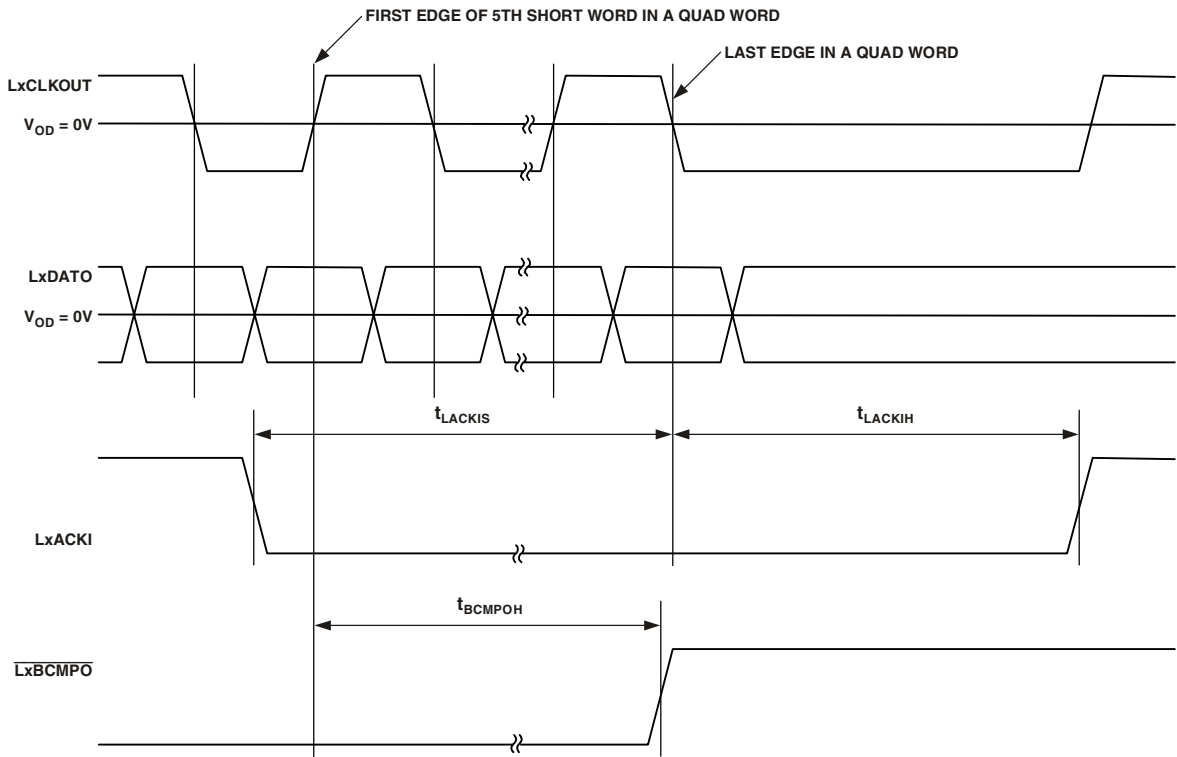
Figure 21. Link Ports—Transmission End and Stops
