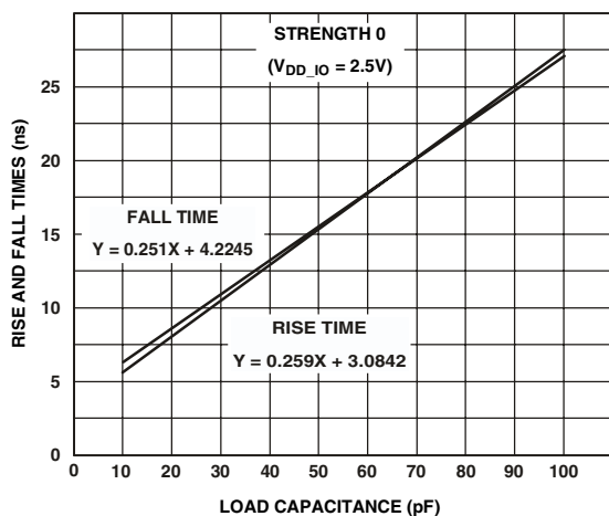
Figure 36. Typical Output Rise and Fall Time (10%–90%, V_{DD\_IO} = 2.5V ) vs. Load Capacitance at Strength 0
