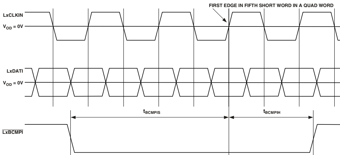
Figure 23. Link Ports—Last Received Quad Word
