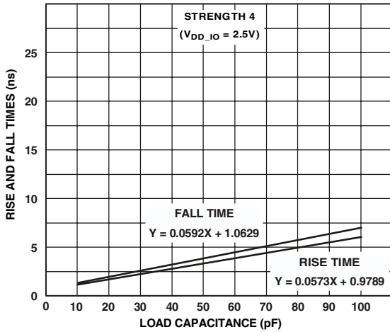
Figure 40. Typical Output Rise and Fall Time (10%–90%, V_{DD\_IO} = 2.5 V ) vs. Load Capacitance at Strength 4
