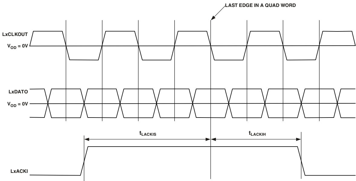
Figure 22. Link Ports—Back to Back Transmission
