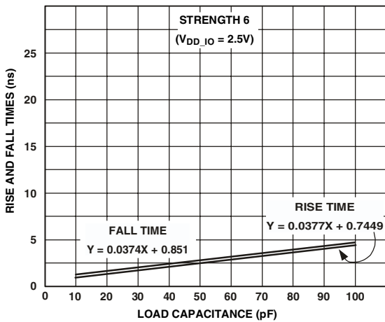
Figure 42. Typical Output Rise and Fall Time (10%–90%, V_{DD\_IO} = 2.5 V ) vs. Load Capacitance at Strength 6
