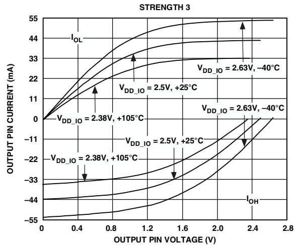
Figure 28. Typical Drive Currents at Strength 3
