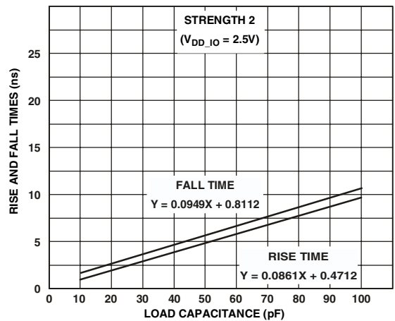
Figure 38. Typical Output Rise and Fall Time (10%–90%, V_{DD\_IO} = 2.5V ) vs. Load Capacitance at Strength 2
