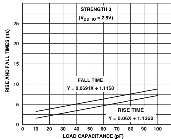
Figure 39. Typical Output Rise and Fall Time (10%–90%, V_{DD\_IO} = 2.5V ) vs. Load Capacitance at Strength 3
