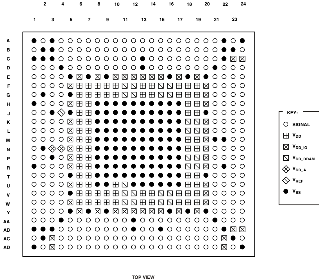
Figure 45. 576-Ball BGA_ED Pin Configurations 1 (Top View, Summary)
