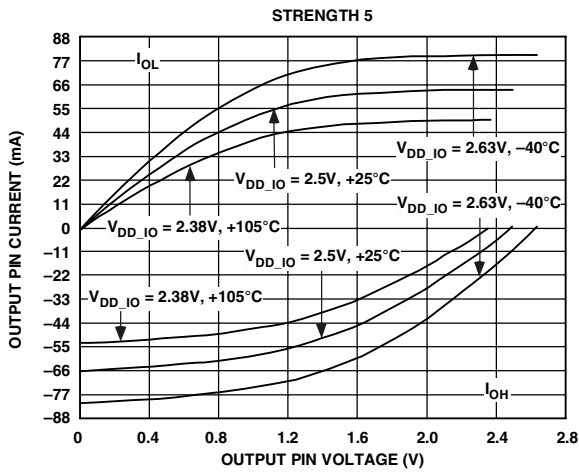
Figure 30. Typical Drive Currents at Strength 5
