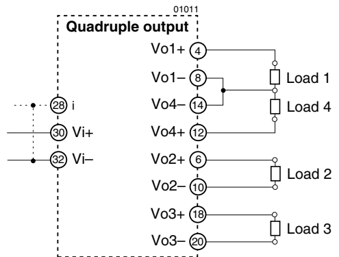
Fig. 6 Common ground configuration of output 1 with 4 and independent configuration of output 2 and 3
