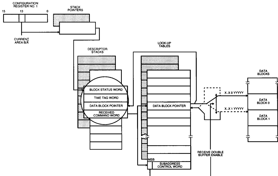
FIGURE 29. RT MEMORY MANAGEMENT: SUBADDRESS DOUBLE BUFFERING MODE
