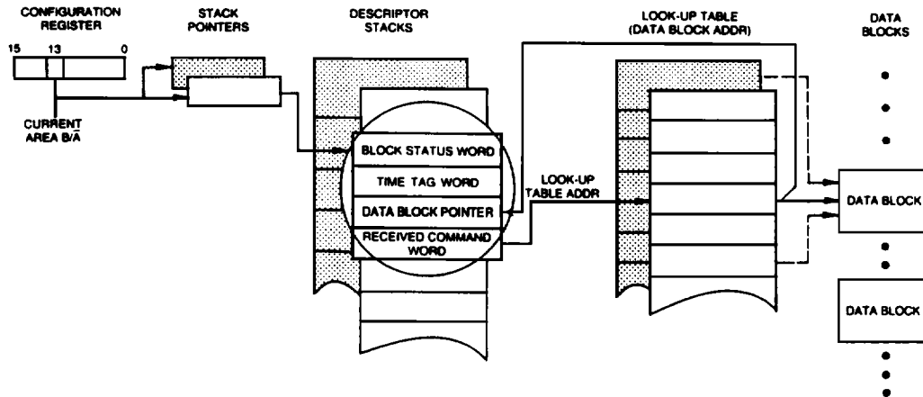
FIGURE 27. RT MEMORY MANAGEMENT: SINGLE MESSAGE MODE
