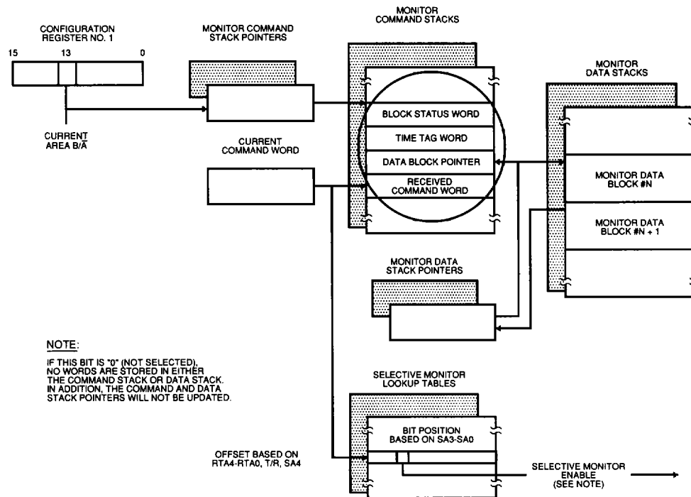
FIGURE 31. SELECTIVE MESSAGE MONITOR MEMORY MANAGEMENT
