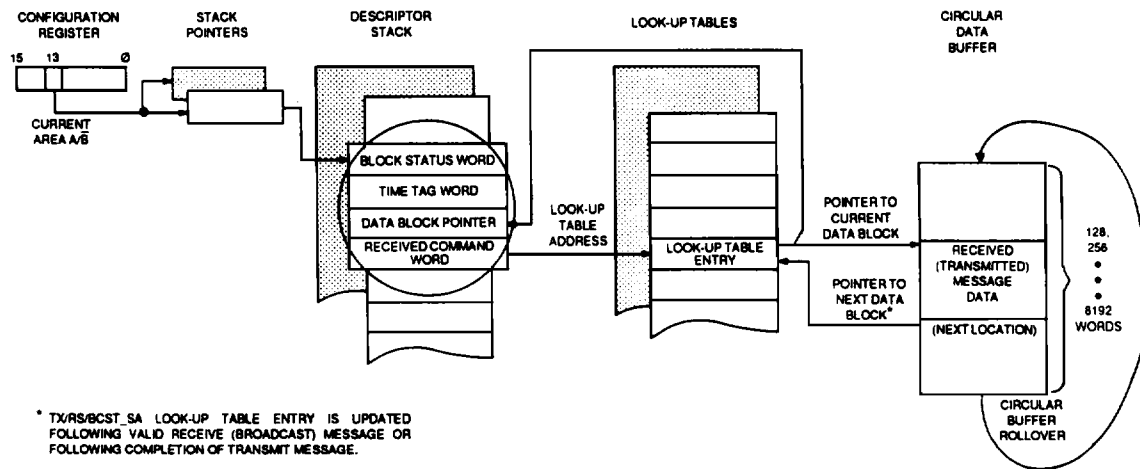
FIGURE 28. RT MEMORY MANAGEMENT: CIRCULAR BUFFER MODE
