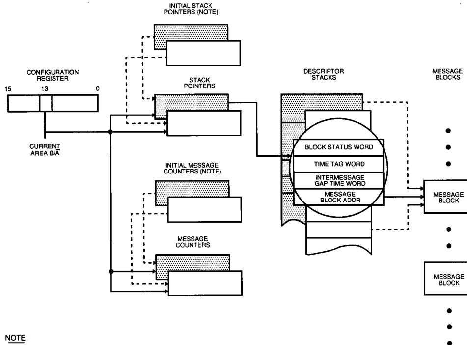
FIGURE 25. BC MODE MEMORY MANAGEMENT
