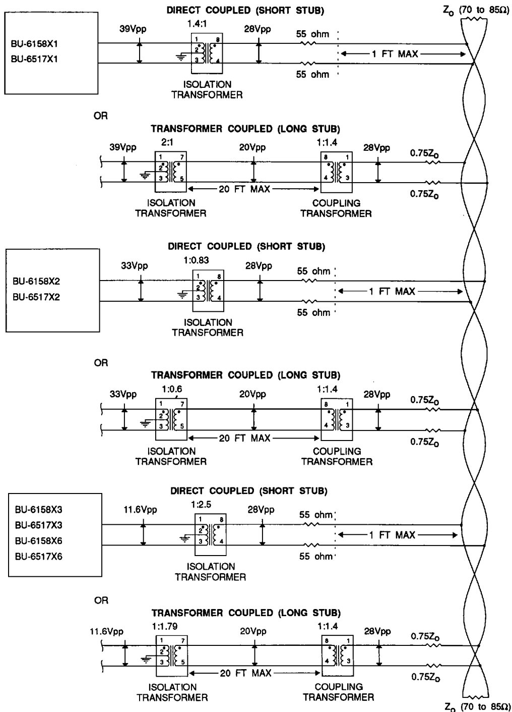
FIGURE 41. BU-65170/61580 INTERFACE TO A 1553 BUS
