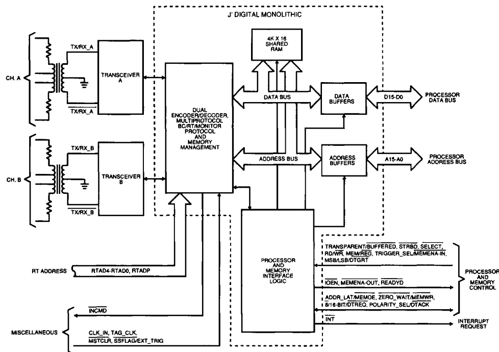
FIGURE1. BU-61580/65170 BLOCK DIAGRAM
