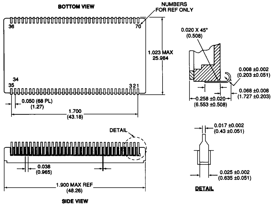
FIGURE 44. BU-65170/61580JX, 70-PIN J-LEAD PACKAGE, MECHANICAL OUTLINE
