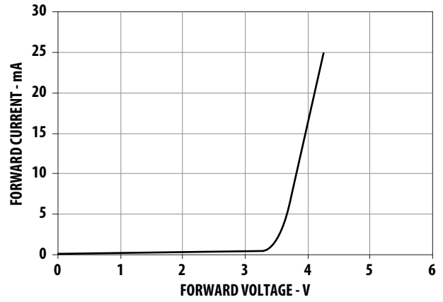
Figure 14. Forward Voltage Vs Current (Segment)
