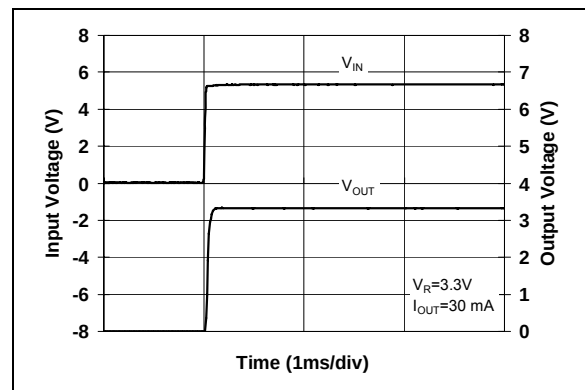
FIGURE 2-35: Startup Response.
