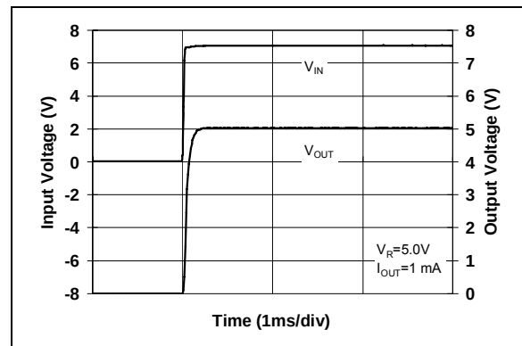
FIGURE 2-36: Startup Response.
