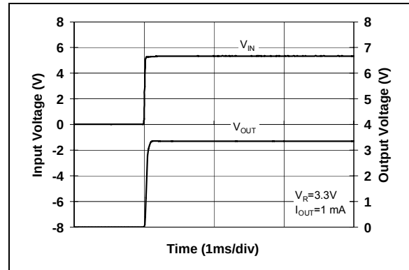
FIGURE 2-34: Startup Response.
