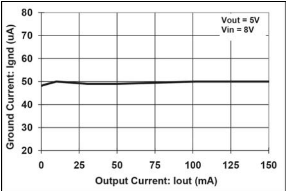
FIGURE 2-52: PSRR 5V @ 30 mA.
