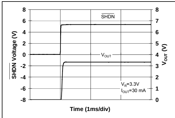
FIGURE 2-43: SHDN Response.
