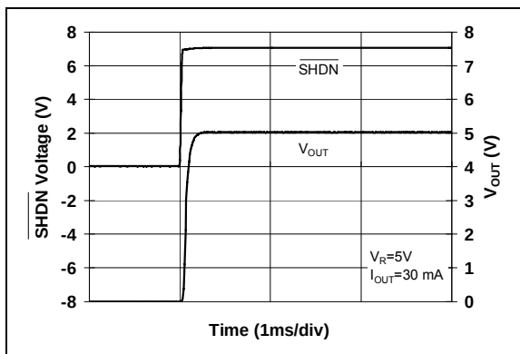
FIGURE 2-44: SHDN Response.
