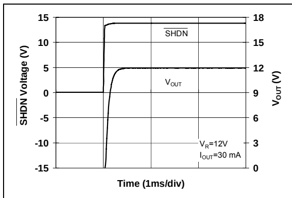
FIGURE 2-45: SHDN Response.
