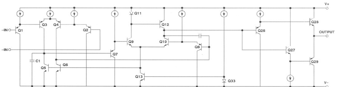
Figure 1. Simplified Schematic (1/4 Shown)
