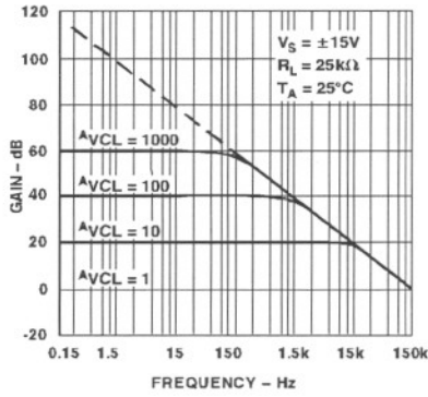
TPC 1. Closed-Loop Gain vs. Frequency
