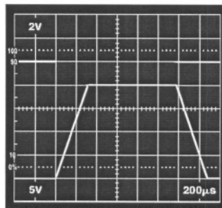
TPC 8. Large-Signal Transient Response
