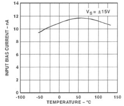
TPC 3. Input Bias Current vs. Temperature
