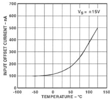
TPC 2. Input Offset Current vs. Temperature
