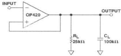
Figure 2. Small-Signal Transient Response
