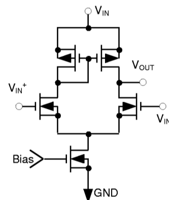
Figure 5 Error amplifier
