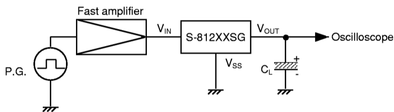
Figure 8 Measuring circuit
