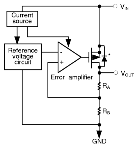
Figure 4 Reference block diagram
