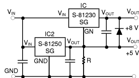
Figure 17 Dual power source
