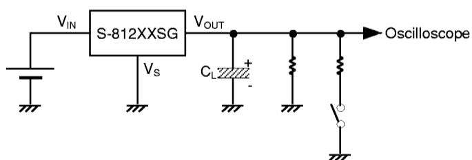
Figure 10 Measuring circuit
