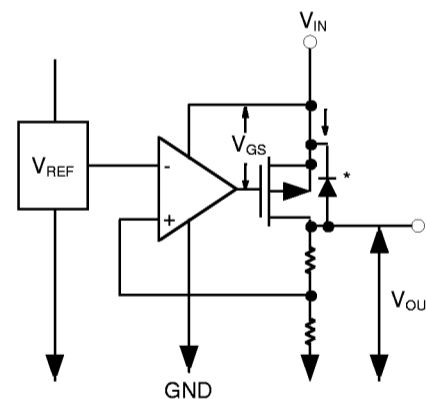
Figure 5 Error amplifier
