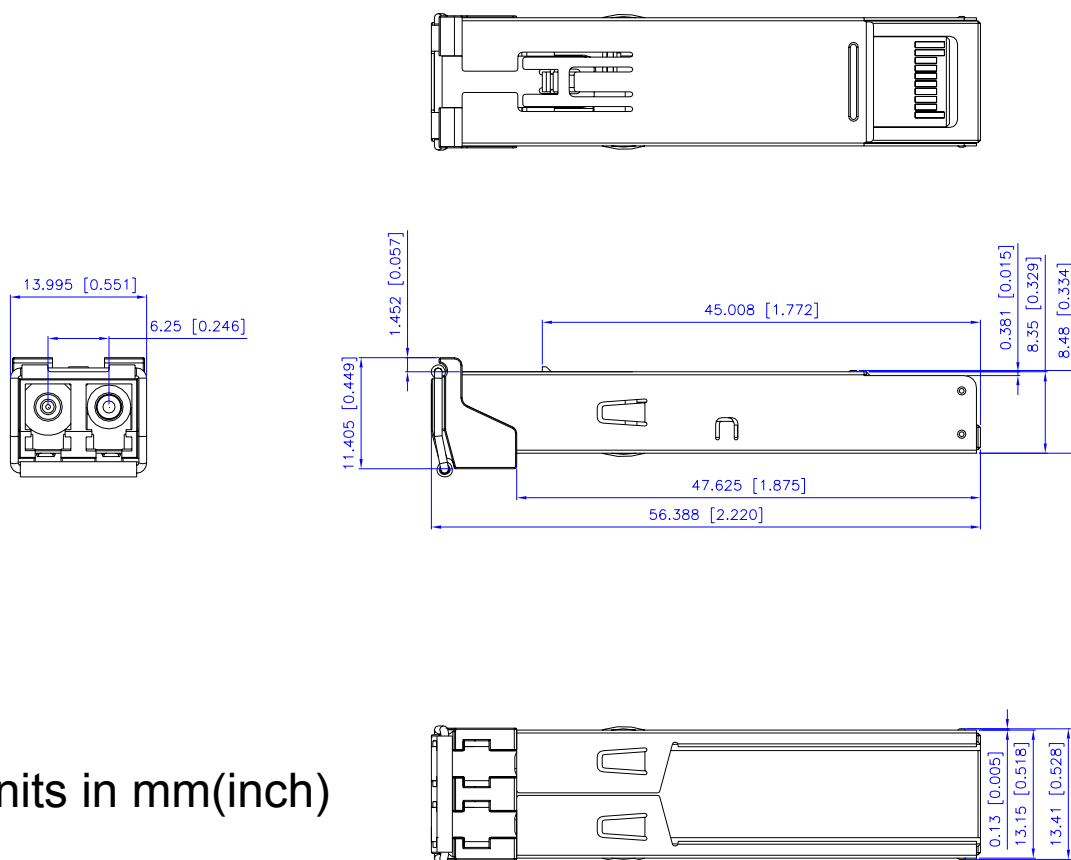
Figure 5, Mechanical Design Diagram of the SFP
