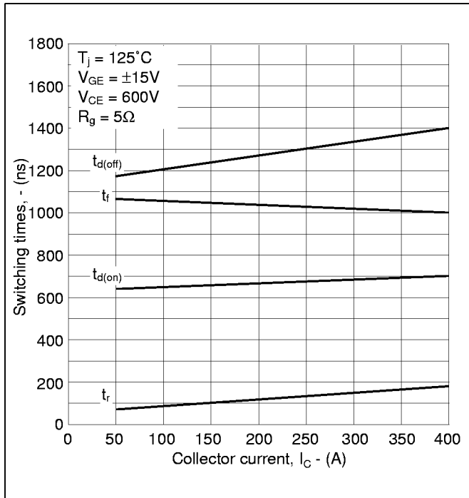
Fig. 14 Typical switching characteristics
