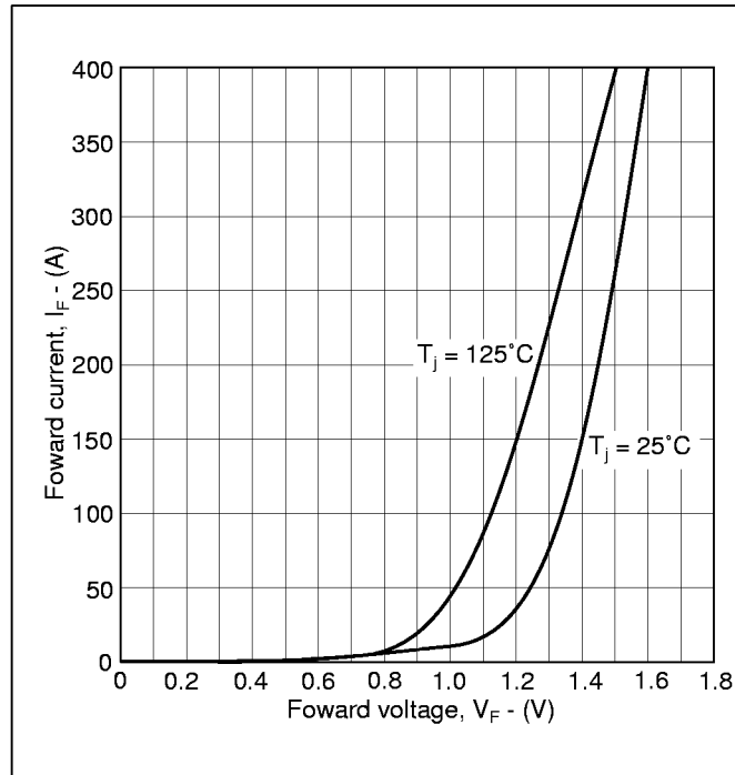
Fig. 15 Diode typical forward characteristics
