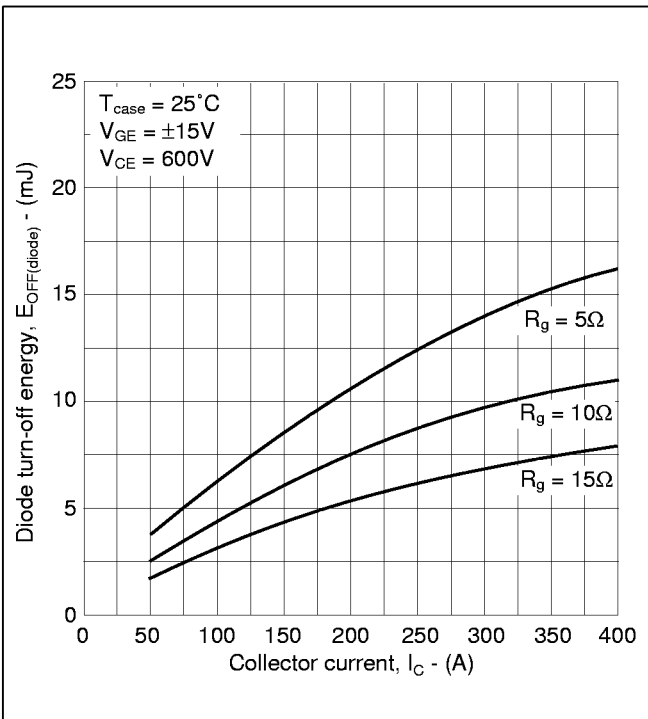
Fig.12 Typical diode turn-off energy vs collector current
