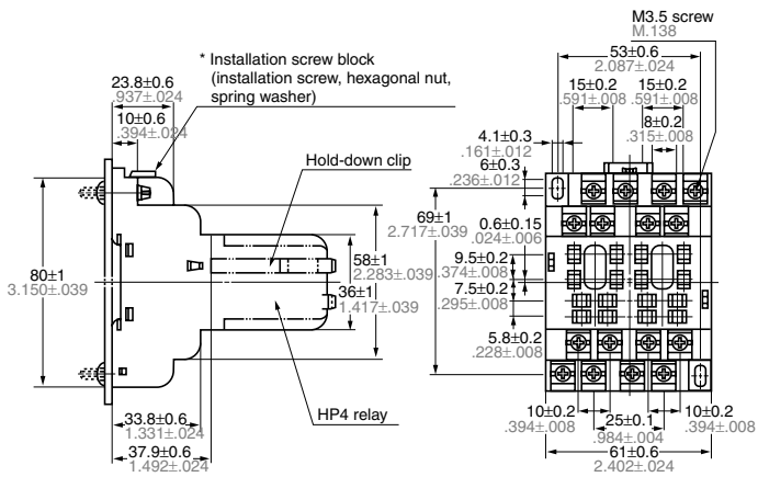
External dimensions
