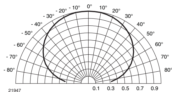
Fig. 10 - Directivity
