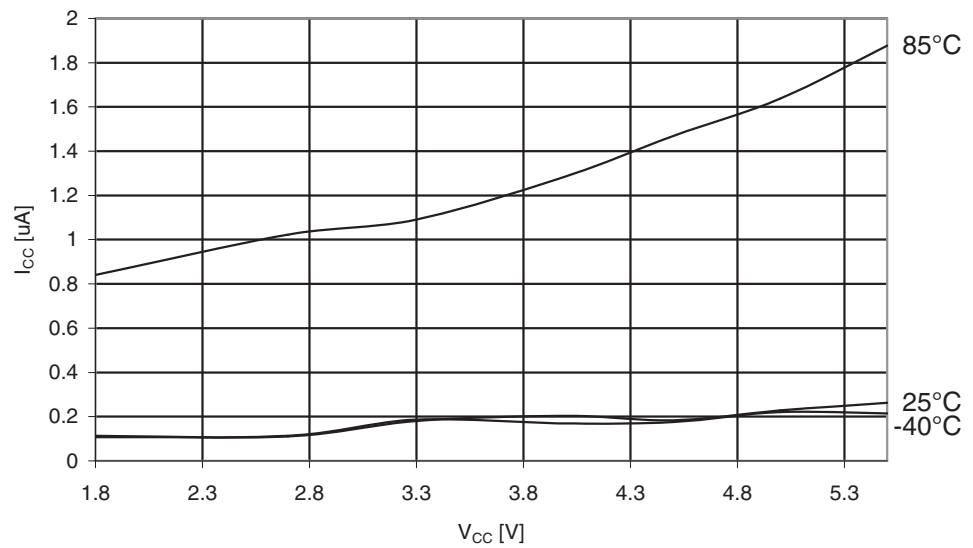
Figure 29-195. ATmega325PA: Power-down Supply Current vs. V_{CC} (Watchdog Timer Disabled)
