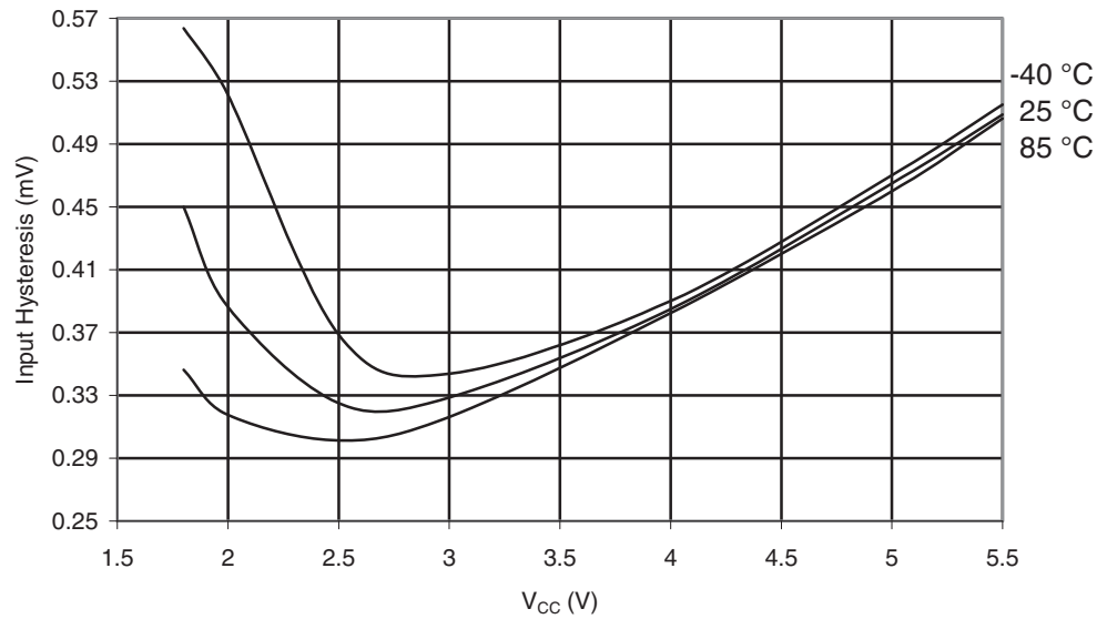
Figure 29-220. ATmega325PA: I/O Pin Input Hysteresis vs. V_{CC}
