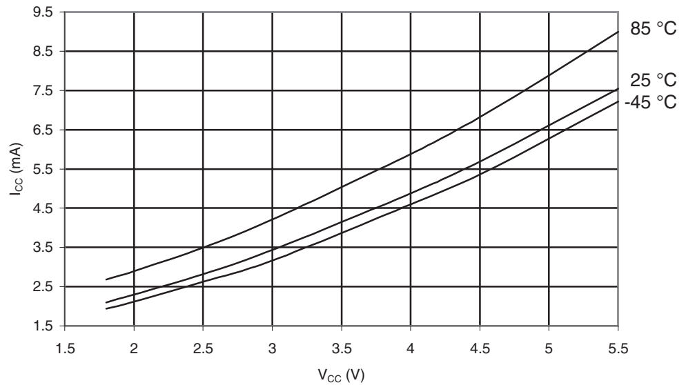
Figure 29-496. ATmega6450A: Idle Supply Current vs. V_{CC} (32kHz Watch Crystal)
