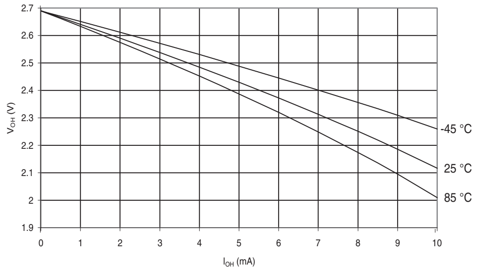
Figure 29-388. ATmega645A: I/O Pin Output Voltage vs. Source Current, Ports A, C, D, E, F, G ( V_{CC} = 2.7V )
