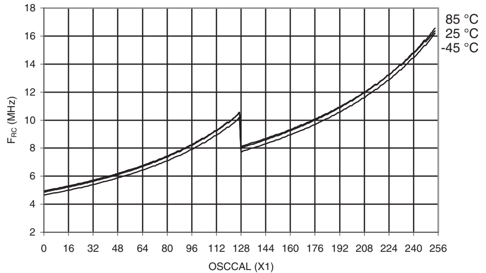
Figure 29-536. ATmega6450A: Calibrated 8MHz RC Oscillator Frequency vs. OSCAL Value
