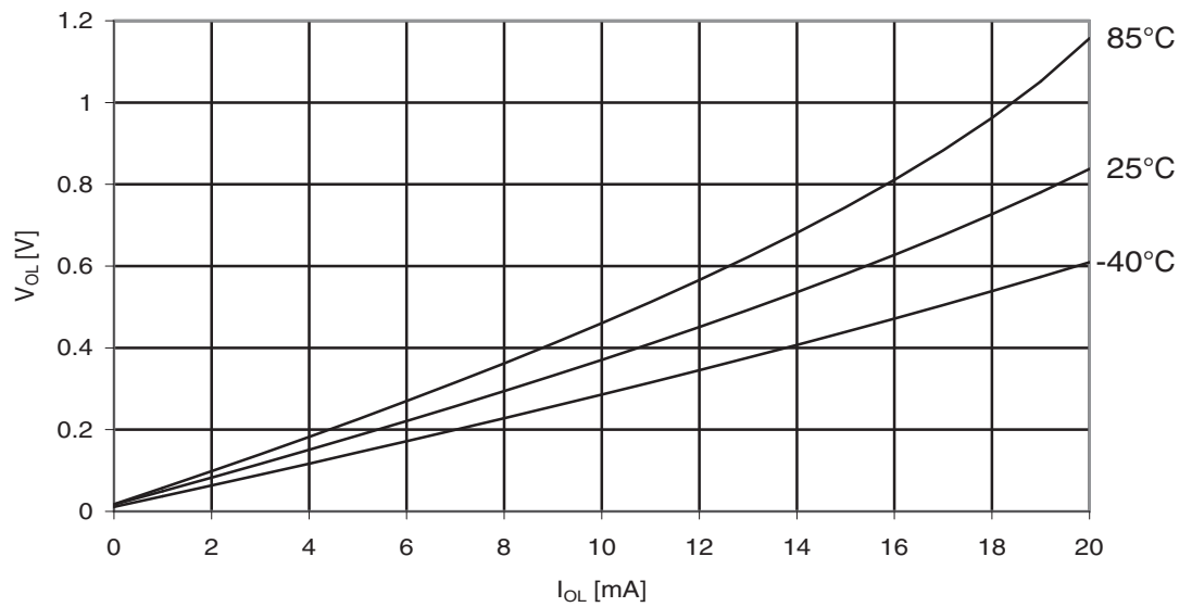
Figure 29-336. ATmega3250PA: I/O Pin Output Voltage vs. Sink Current, Port B ( V_{CC} = 2.7V )
