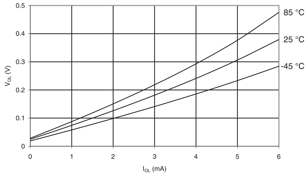
Figure 29-33. ATmega165A: I/O Pin Output Voltage vs. Sink Current, Port B ( V_{CC} = 1.8V )
