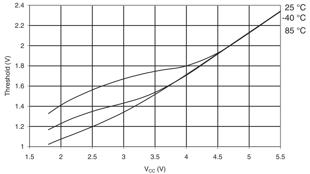
Figure 29-341. ATmega3250PA: Reset Input Threshold Voltage vs. V_{CC} ( V_{IH} , Reset Pin Read as "1")
