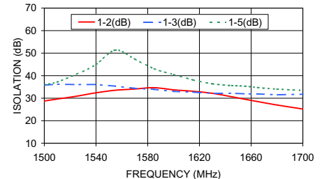
ZB6PD-1700 ISOLATION
