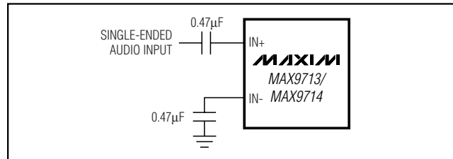
Figure 4. Single-Ended Input
