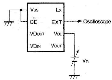
Test Circuit 3
