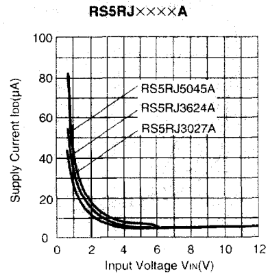
13) Supply Current vs. Input Voltage
