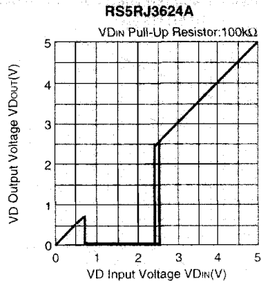
12) VD Output Voltage vs. VD Input Voltage
