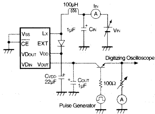
Test Circuit 6
