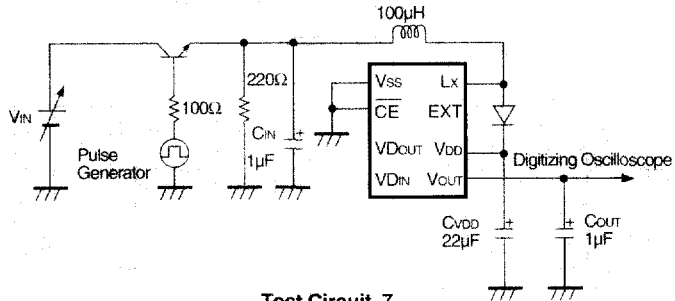
Test Circuit 7
