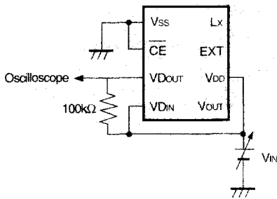
Test Circuit 2
