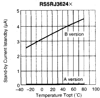
14) Stand-by Current vs. Temperature
