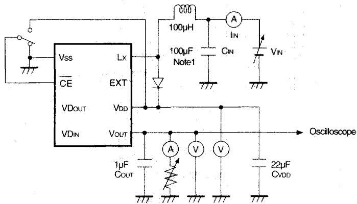
Test Circuit 1
