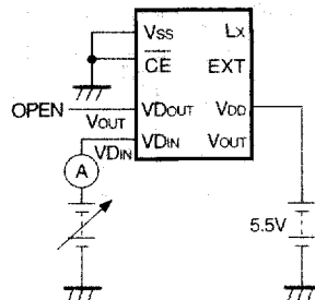
Test Circuit 5
