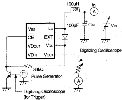
Test Circuit 4
