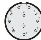
Disposition 18-11 11 contacts taille/size 16
