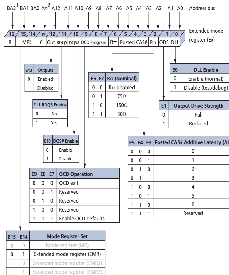
Figure 40: Extended Mode Register Definition
