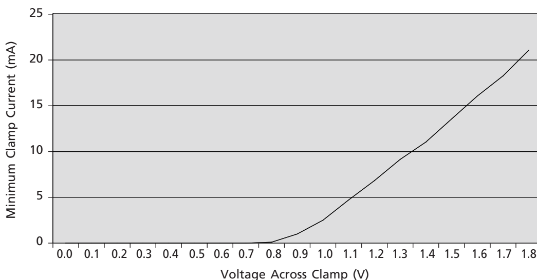
Figure 22: Input Clamp Characteristics
