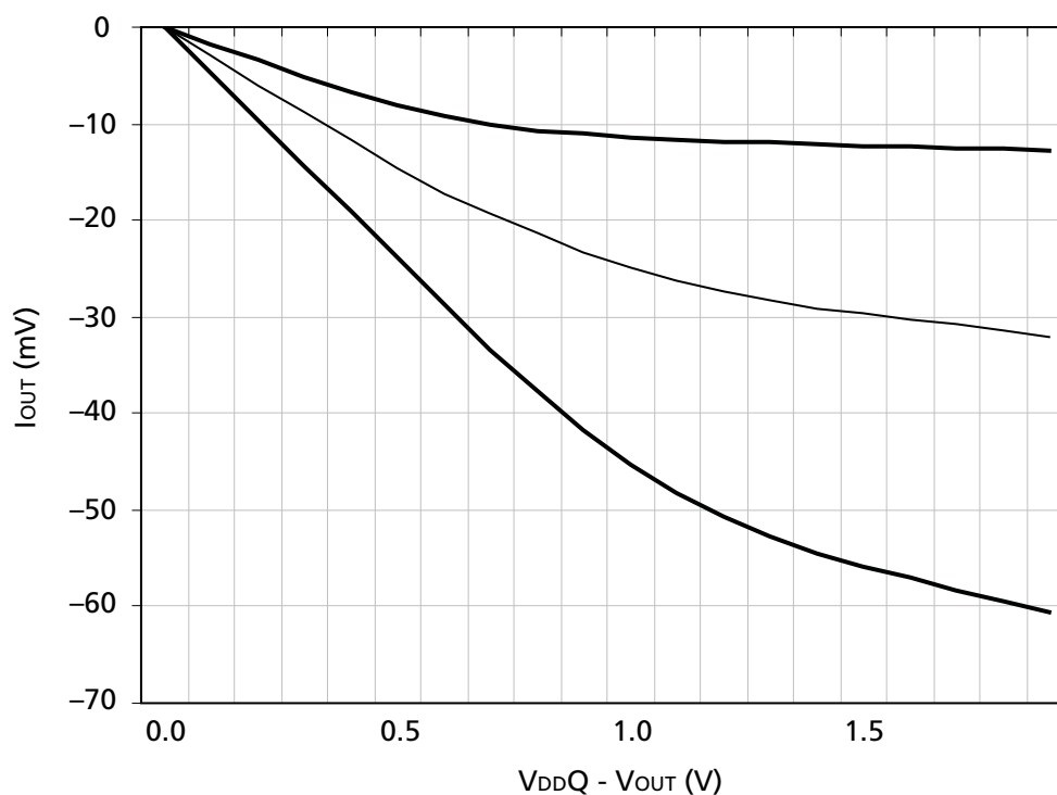
Figure 21: Reduced Strength Pull-Up Characteristics
