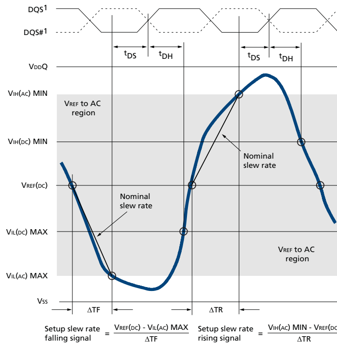
Figure 29: Nominal Slew Rate for t_{DS}
