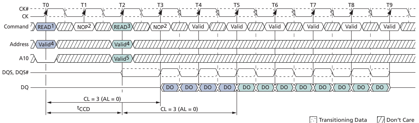
Figure 50: READ Interrupted by READ
