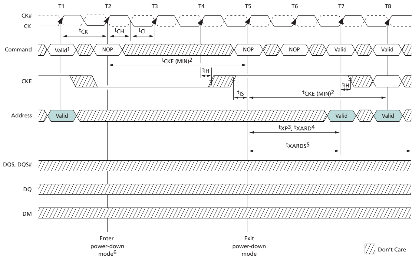
Figure 71: Power-Down
