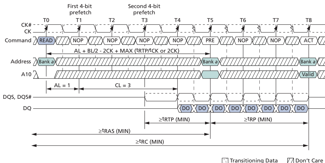
Figure 53: READ-to-PRECHARGE – BL = 8
