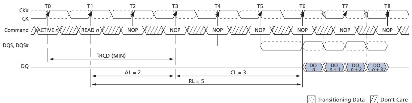
Figure 41: READ Latency
