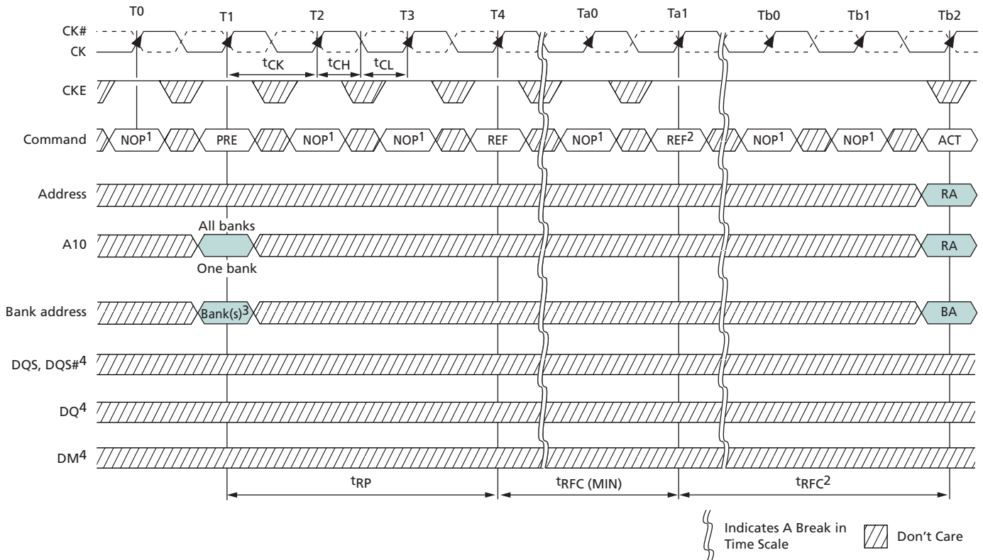
Figure 69: Refresh Mode
