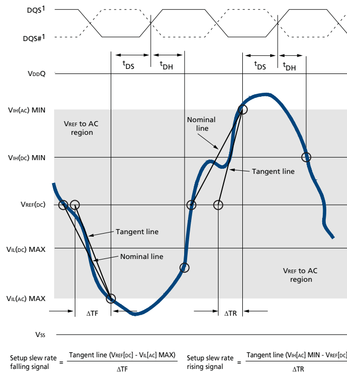
Figure 30: Tangent Line for t_{DS}
