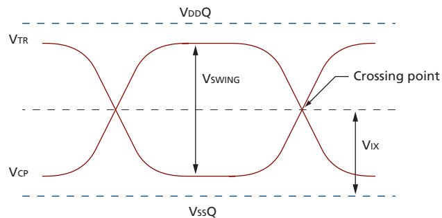
Figure 36: AC Input Test Signal Waveform (Differential)
