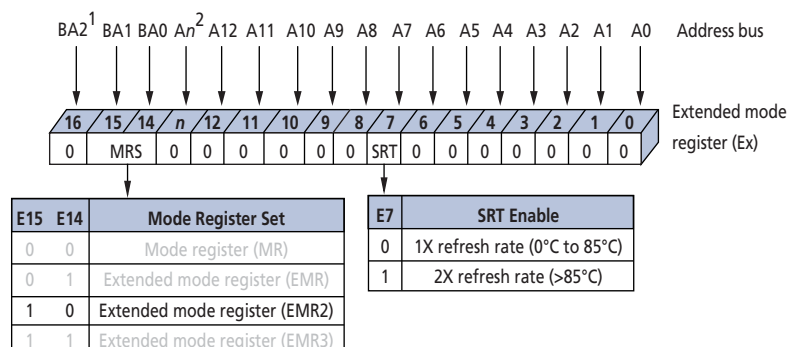
Figure 43: Extended Mode Register 2 (EMR2) Definition
