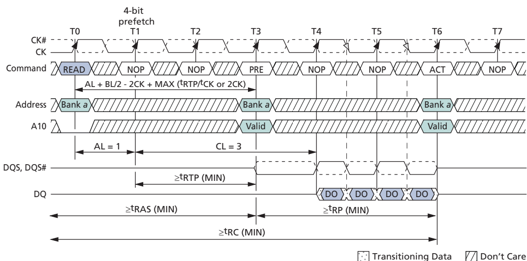
Figure 52: READ-to-PRECHARGE – BL = 4
