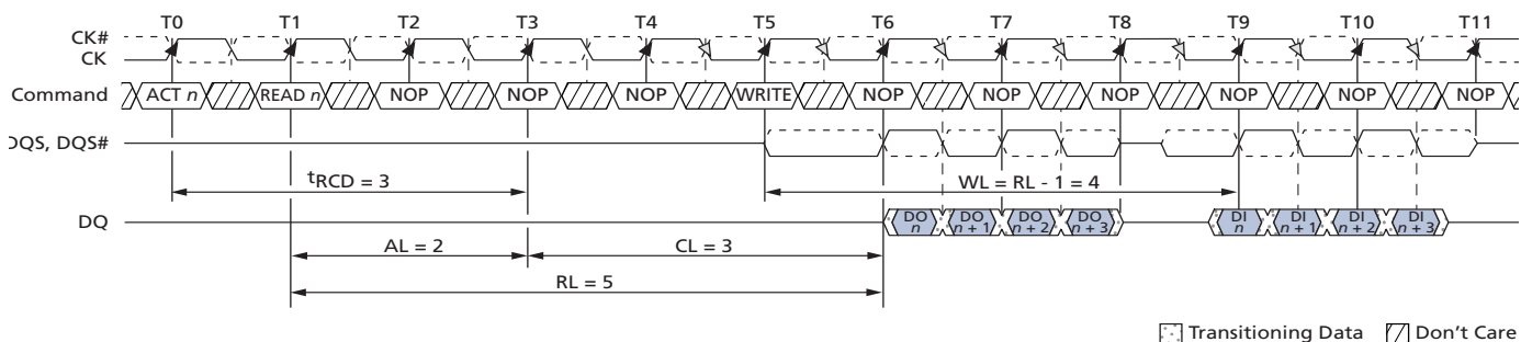
Figure 51: READ-to-WRITE
