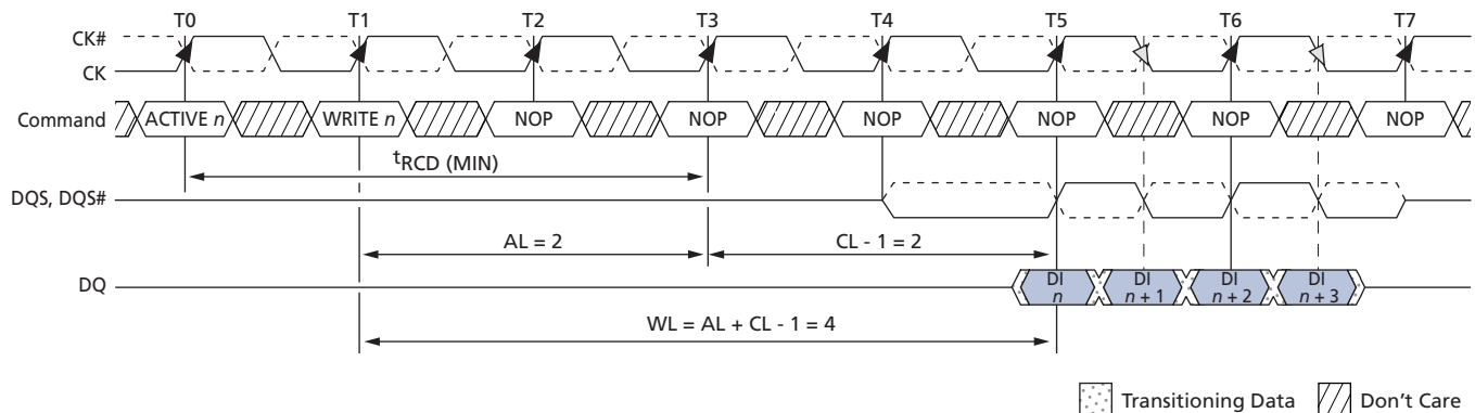
Figure 42: WRITE Latency
