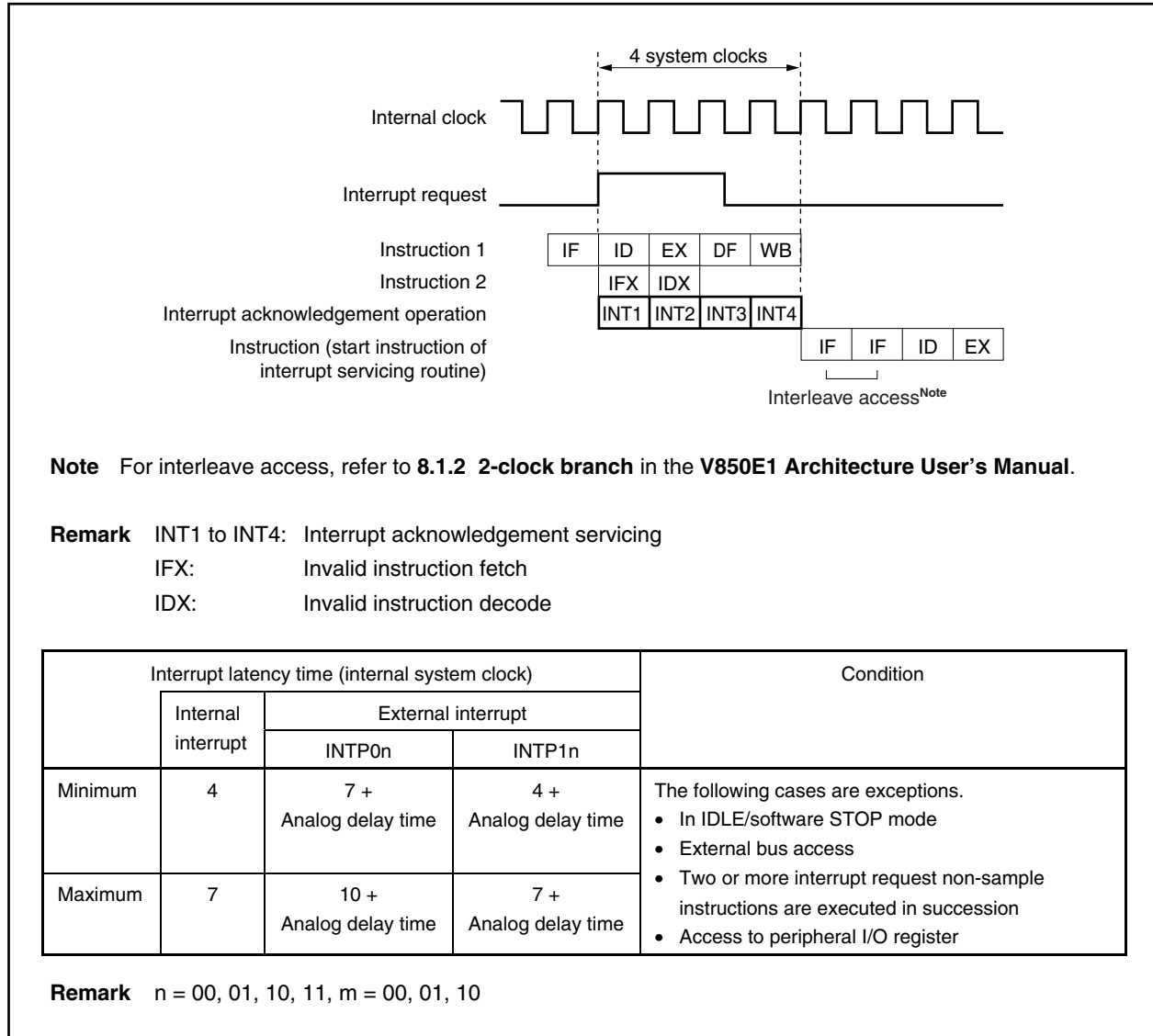
★ Figure 7-14. Pipeline Operation at Interrupt Request Acknowledgement (Outline)
