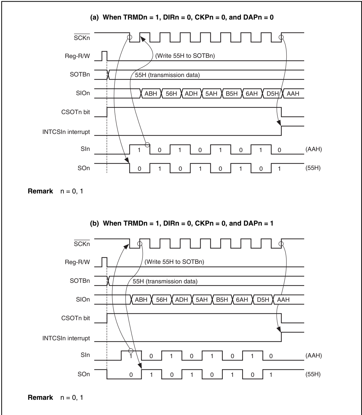
Figure 11-16. Transfer Timing
