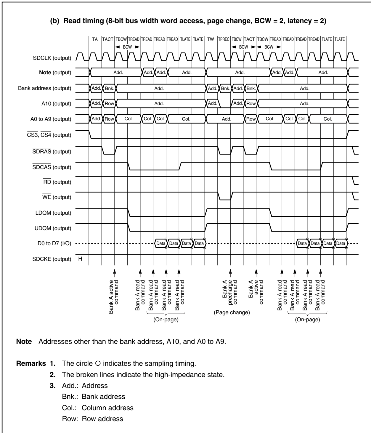
Figure 5-11. SDRAM Access Timing (2/4)
