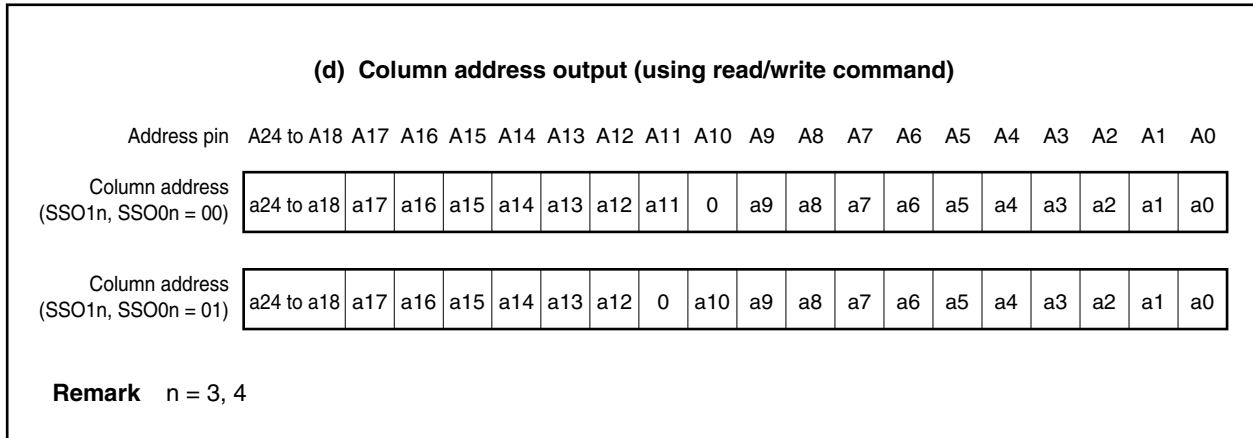
Figure 5-7. Row Address/Column Address Output (2/2)
