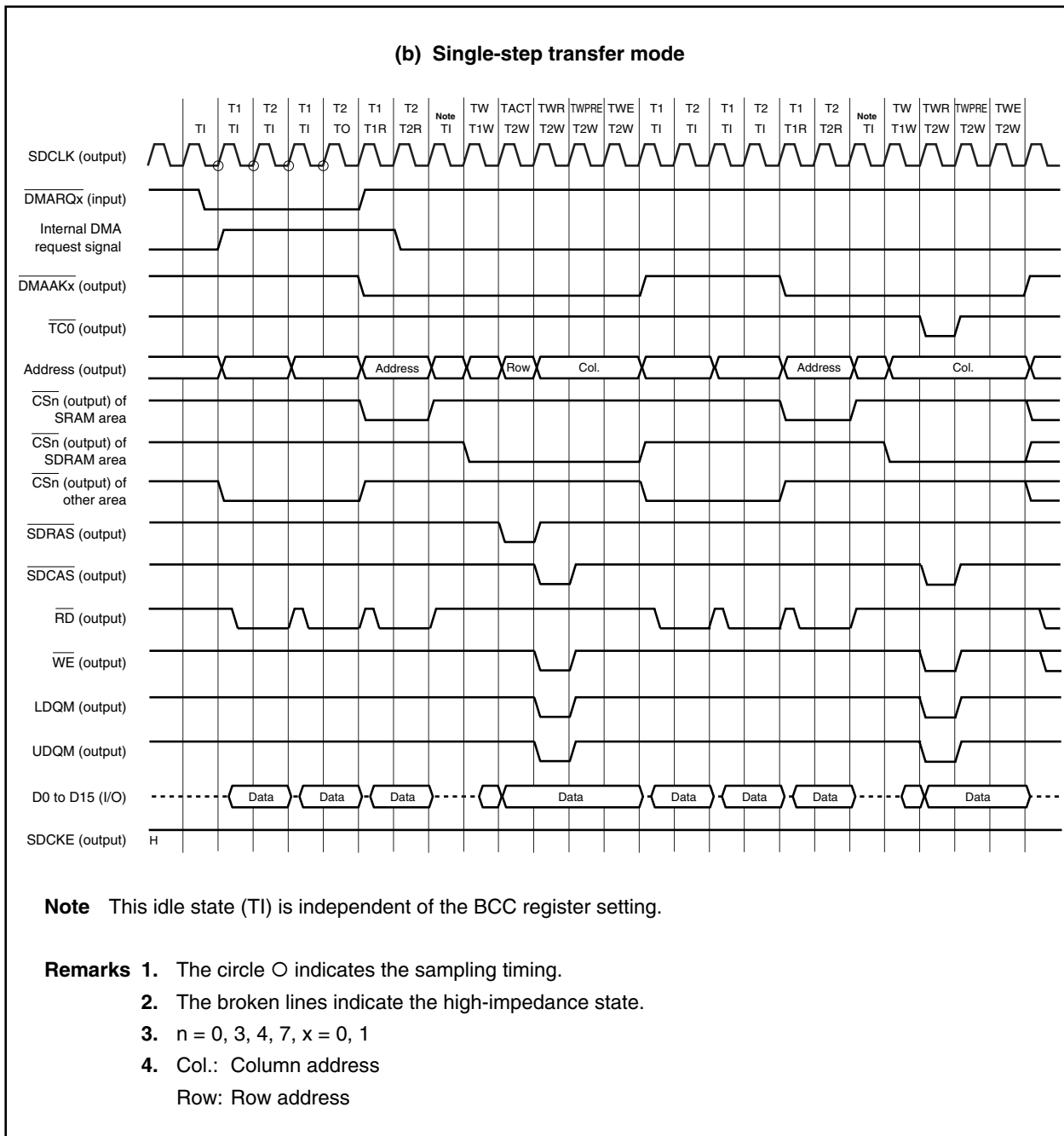
Figure 6-10. Timing of 2-Cycle DMA Transfer (SRAM → SDRAM) (2/3)
