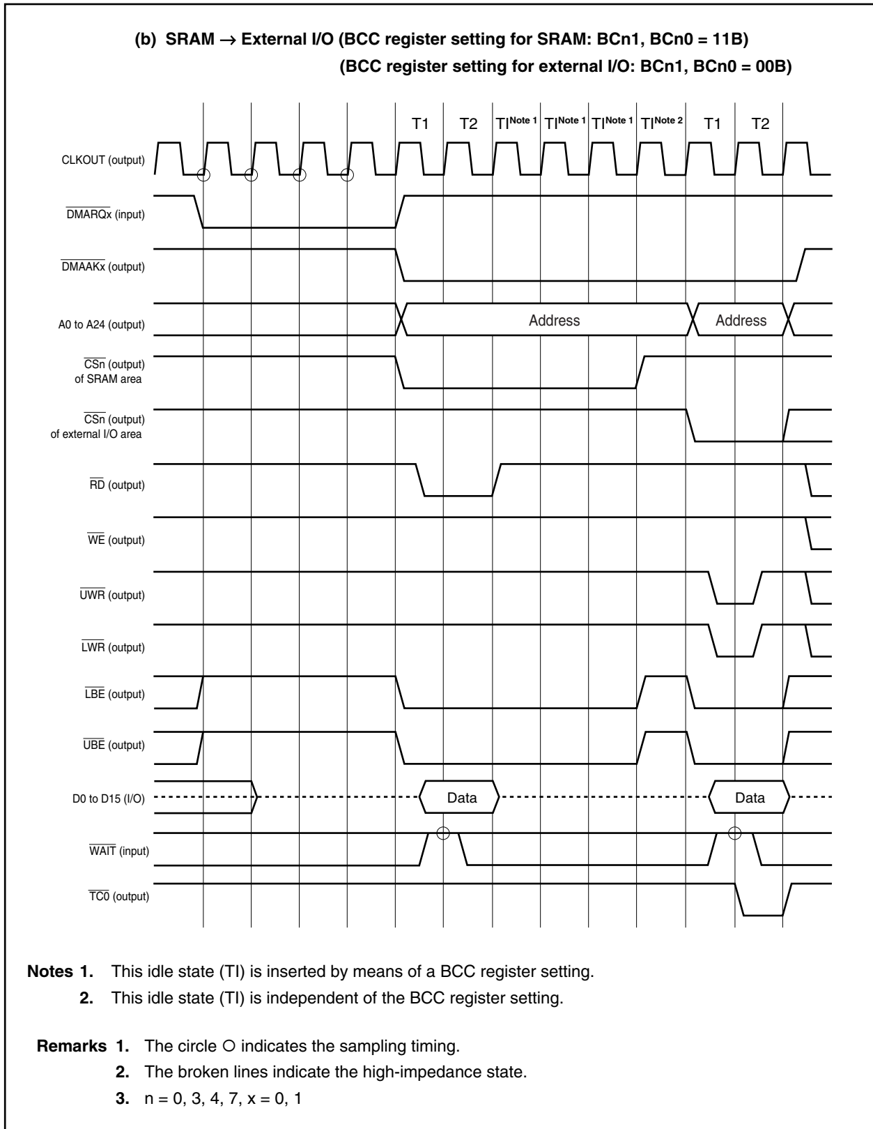
Figure 6-8. Timing of Access to SRAM, External ROM, and External I/O During 2-Cycle DMA Transfer (2/2)
