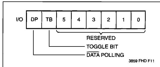
Figure 1. Status Bit Assignment
