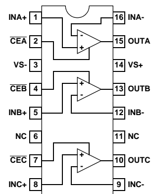
EL5392 [16 LD SOIC (0.150") & QSOP] TOP VIEW
