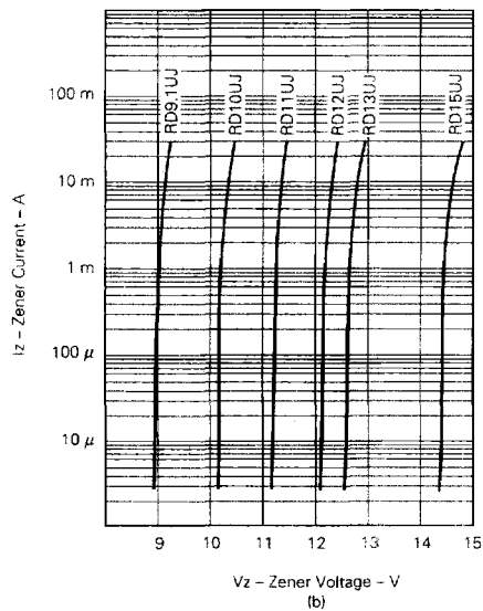
Fig. 2 I_z - V_z CHARACTERISTICS (a to d)
