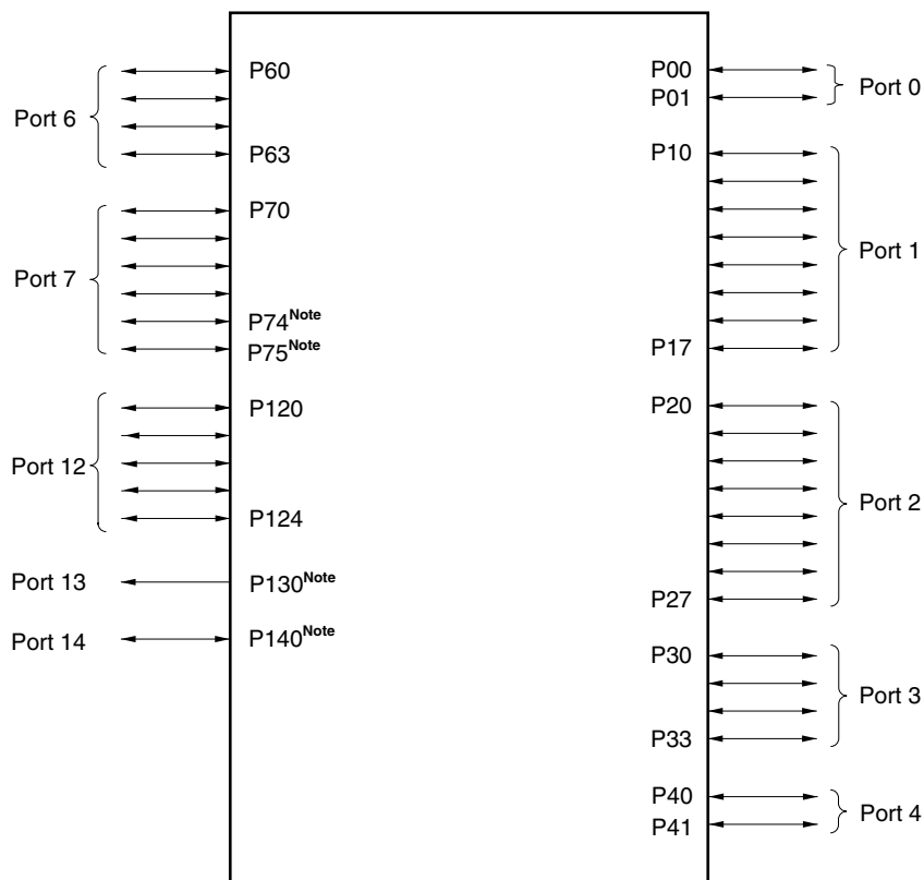
Figure 4-1. Port Types
