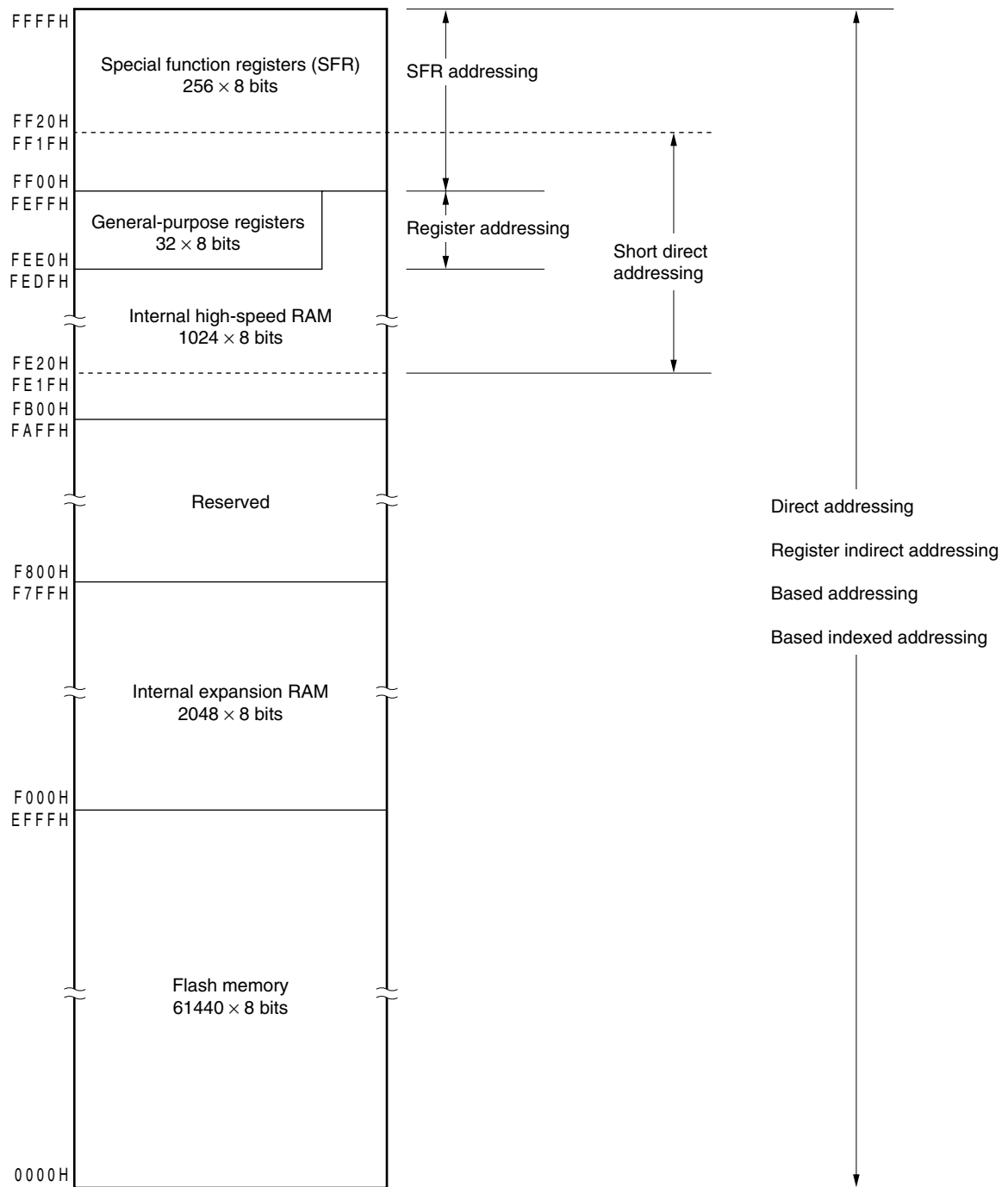
Figure 3-14. Correspondence Between Data Memory and Addressing ( \mu PD78F0515D)
