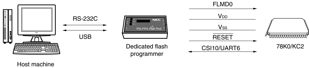
Figure 25-7. Environment for Writing Program to Flash Memory
