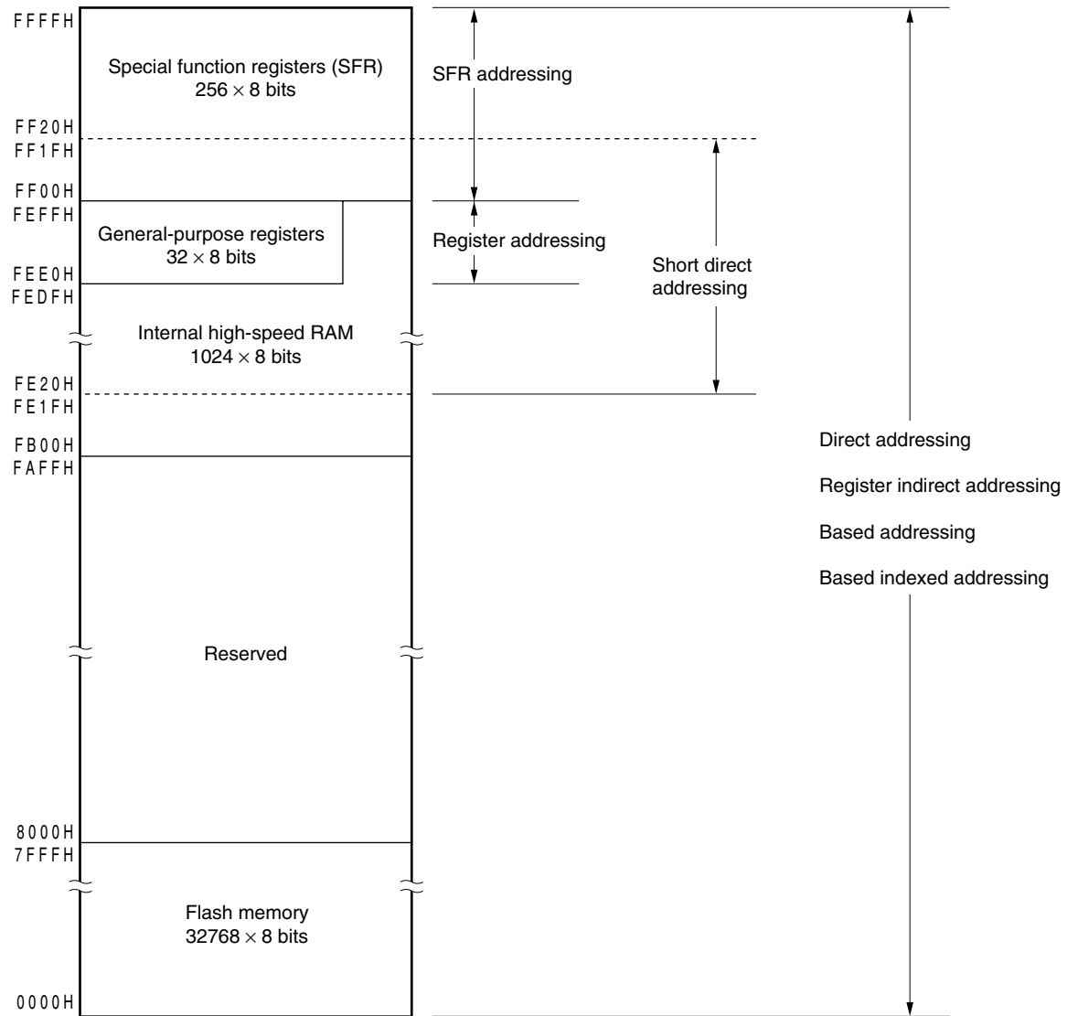
Figure 3-11. Correspondence Between Data Memory and Addressing ( \mu PD78F0513D)
