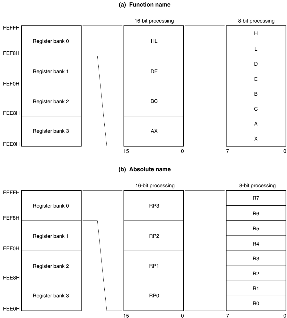
Figure 3-20. Configuration of General-Purpose Registers
