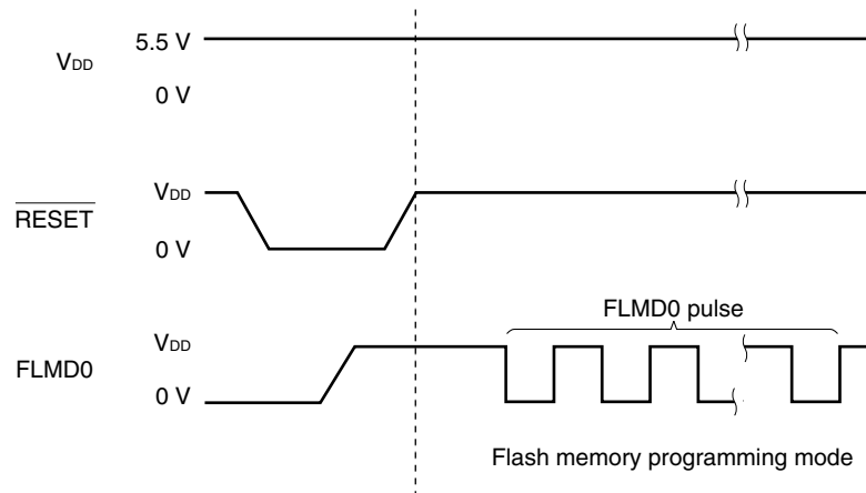
Figure 25-15. Flash Memory Programming Mode
