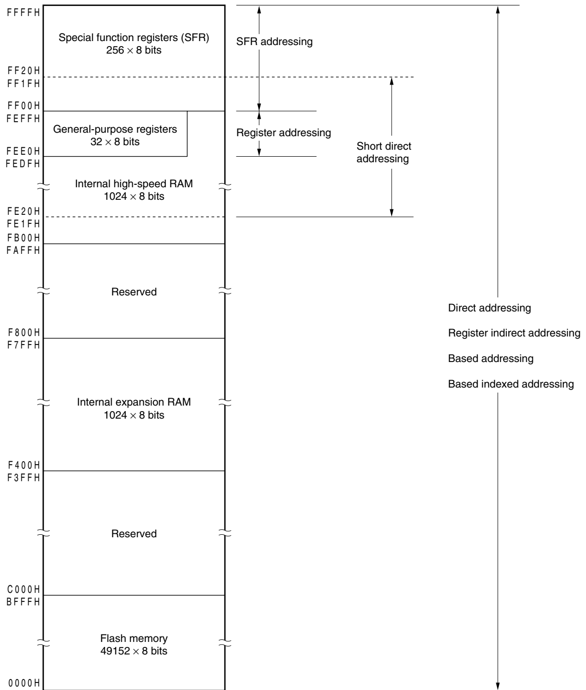
Figure 3-12 . Correspondence Between Data Memory and Addressing ( \mu PD78F0514)
