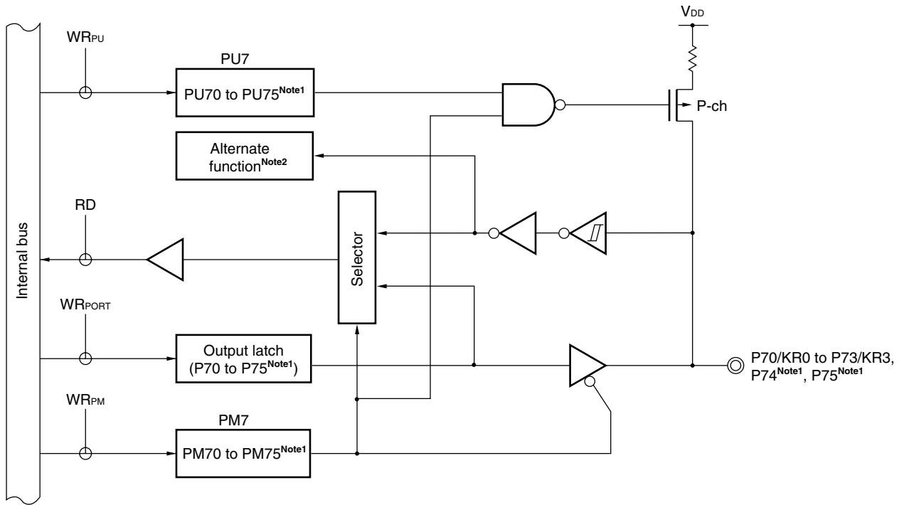
Figure 4-16. Block Diagram of P70 to P75
