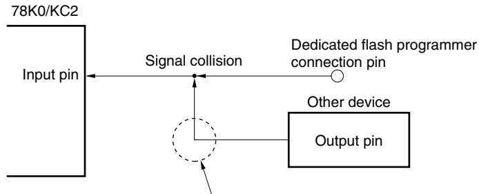
Figure 25-11. Signal Collision (Input Pin of Serial Interface)
