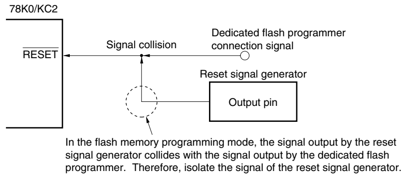
Figure 25-13. Signal Collision ( \overline{\text{RESET}} Pin)
