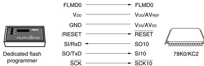
Figure 25-8. Communication with Dedicated Flash Programmer (CSI10)
