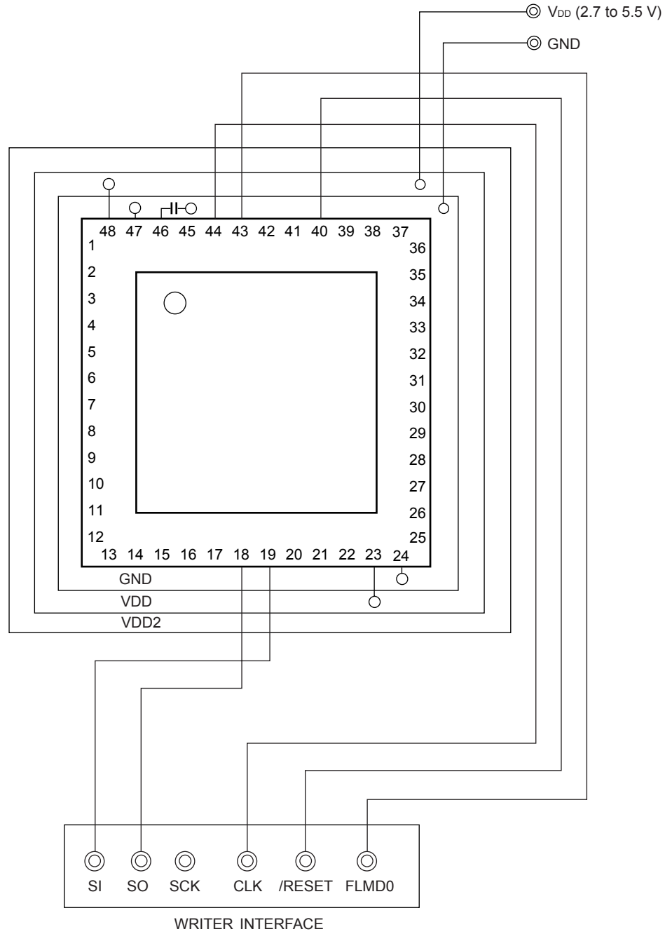
Figure 25-6. Example of Wiring Adapter for Flash Memory Writing in UART (UART6) Mode (48-pin products)
