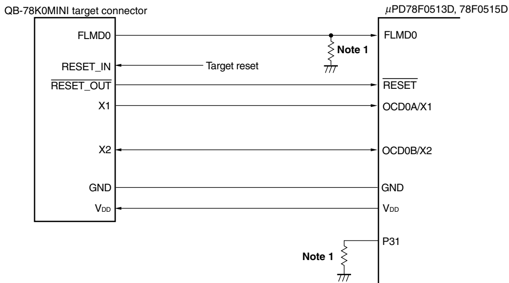
Figure 26-1. Connection Example of QB-78K0MINI and μPD78F0513D, 78F0515D (When OCD0A/X1 and OCD0B/X2 Are Used)
