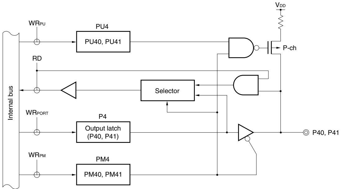
Figure 4-12. Block Diagram of P40, P41
