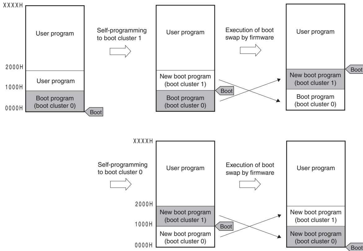
Figure 25-19. Boot Swap Function
