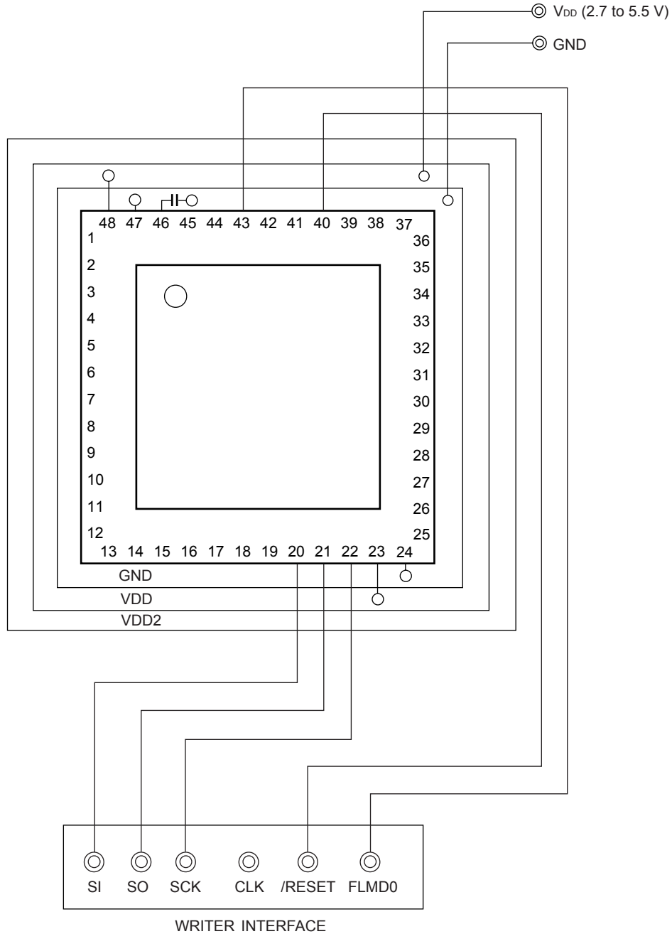
★ Figure 25-5. Example of Wiring Adapter for Flash Memory Writing in 3-Wire Serial I/O (CSI10) Mode (48-pin products)
