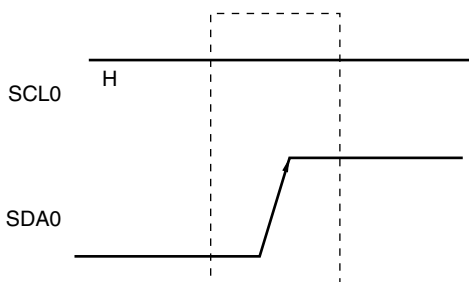
Figure 16-17. Stop Condition
