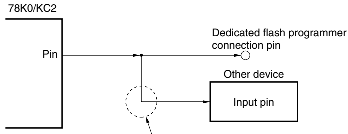
Figure 25-12. Malfunction of Other Device
