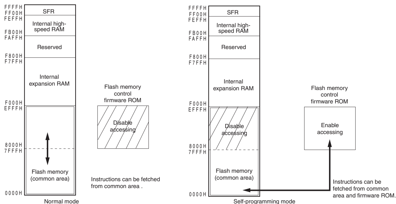
Figure 25-17. Operation Mode and Memory Map for Self-Programming ( \mu PD78F0515)
