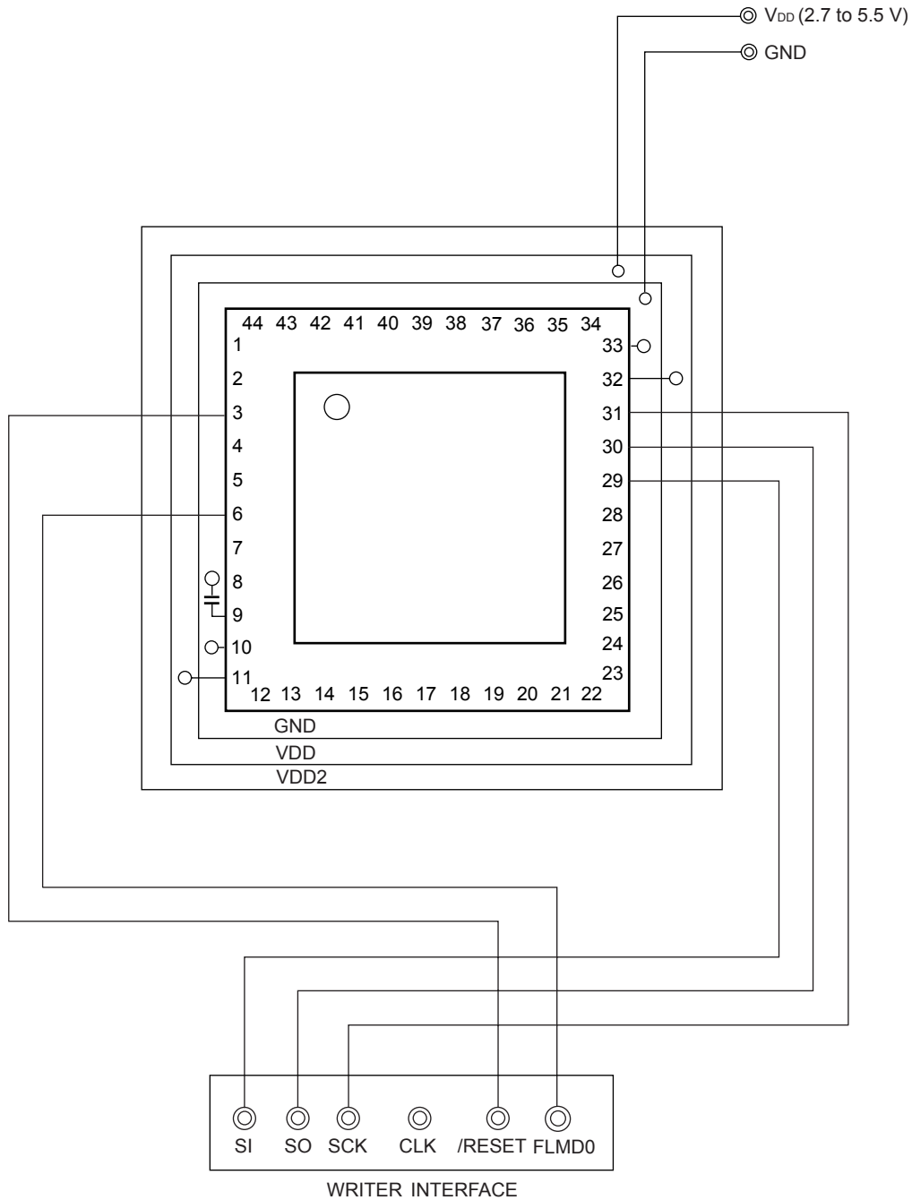
★ Figure 25-3. Example of Wiring Adapter for Flash Memory Writing in 3-Wire Serial I/O (CSI10) Mode (44-pin products)
