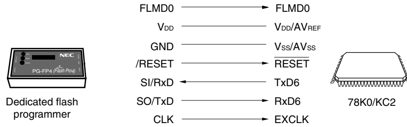
Figure 25-9. Communication with Dedicated Flash Programmer (UART6)
