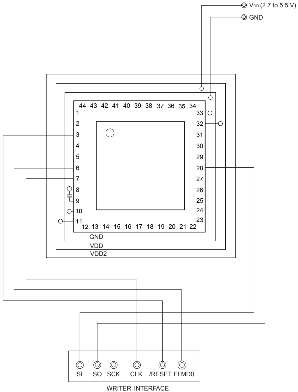
Figure 25-4. Example of Wiring Adapter for Flash Memory Writing in UART (UART6) Mode (44-pin products)
