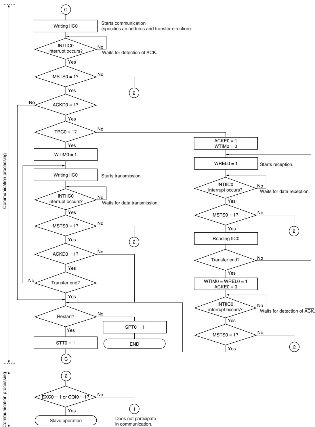
Figure 16-24. Master Operation Flowchart (Multi-Master System) (3/3)
