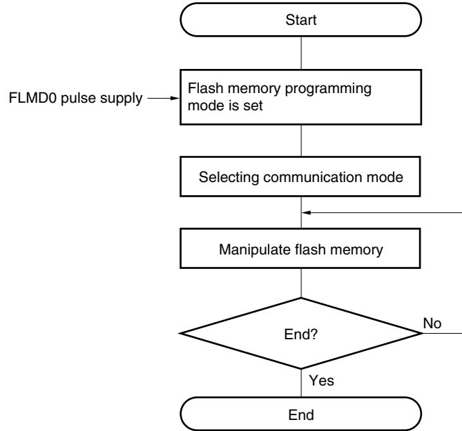
Figure 25-14. Flash Memory Manipulation Procedure
