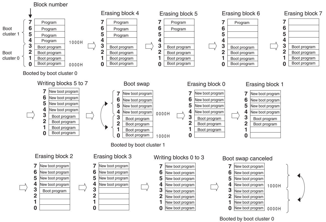
Figure 25-20. Example of Executing Boot Swapping
