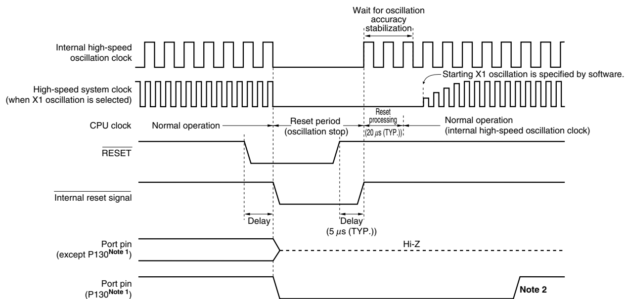
Figure 21-2. Timing of Reset by RESET Input
