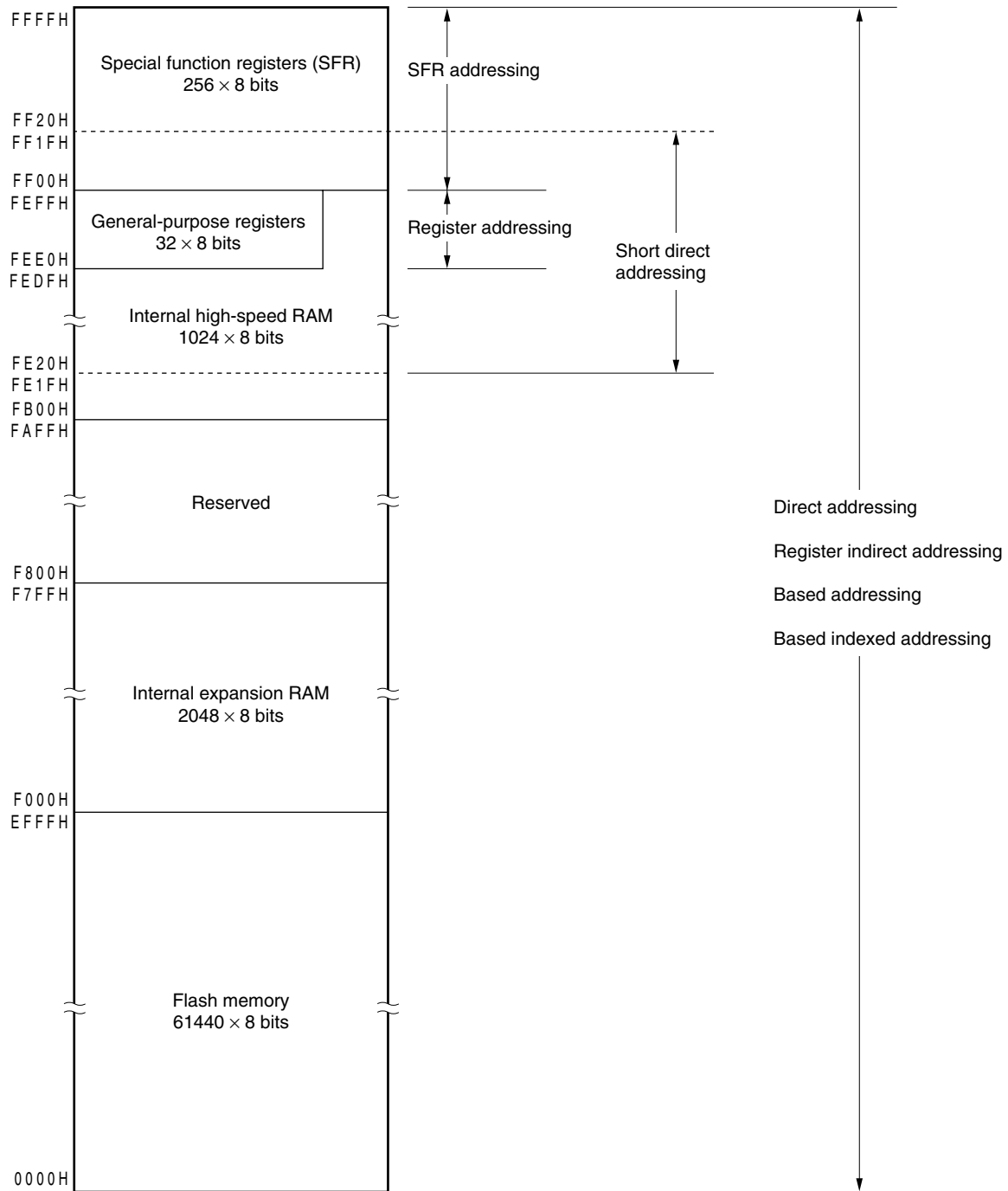
Figure 3-13. Correspondence Between Data Memory and Addressing ( \mu PD78F0515)
