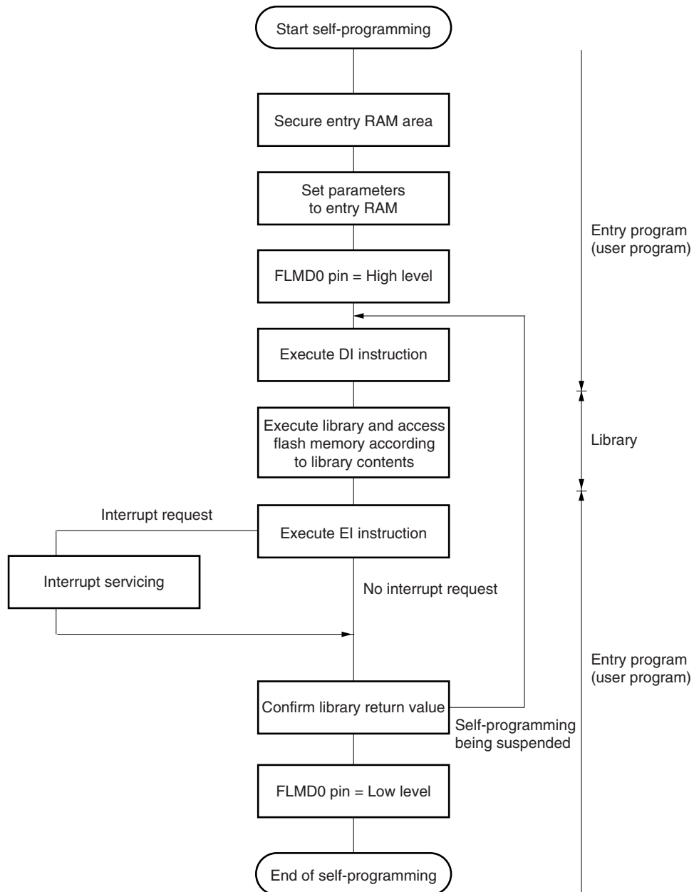
Figure 25-18. Self-Programming Procedure
