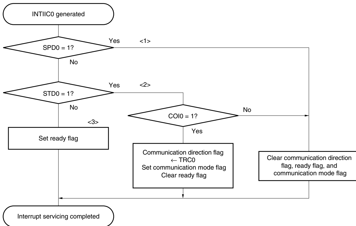
Figure 16-26. Slave Operation Flowchart (2)
