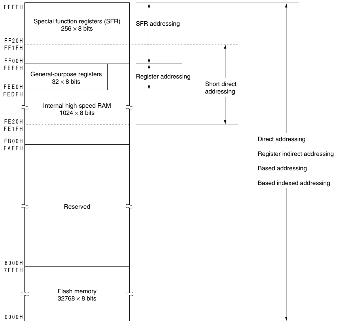
Figure 3-10. Correspondence Between Data Memory and Addressing ( \mu PD78F0513)
