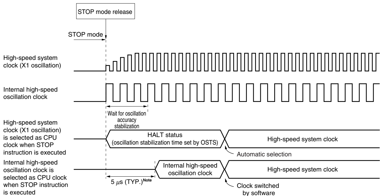
Figure 20-5. Operation Timing When STOP Mode Is Released
