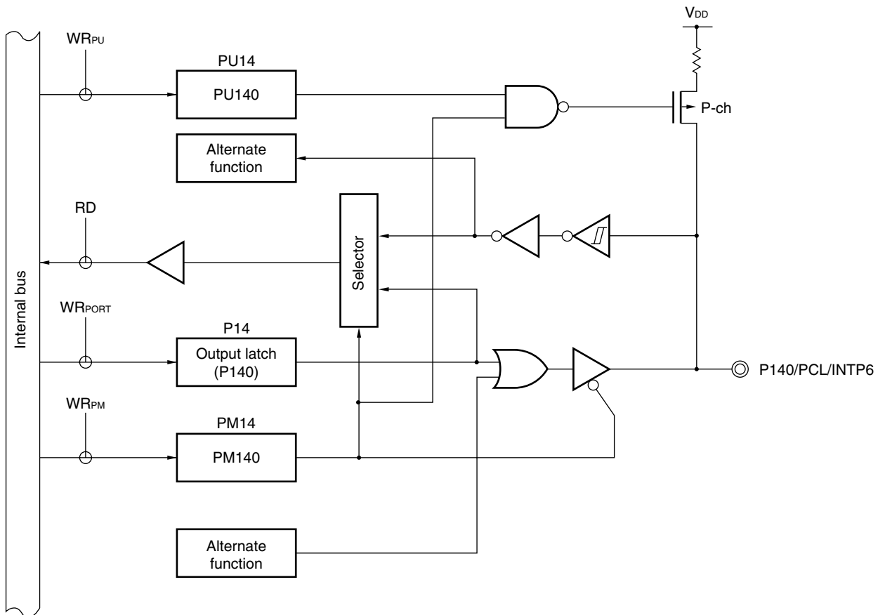
Figure 4-20. Block Diagram of P140
