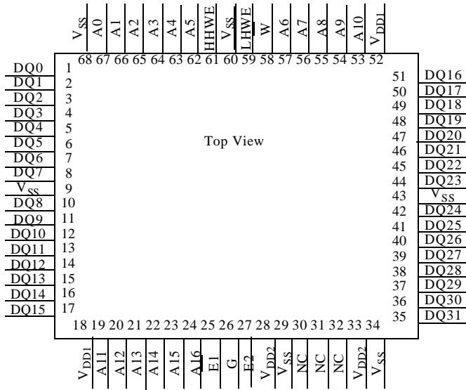
Figure 2. 10ns SRAM Pinout (68)
