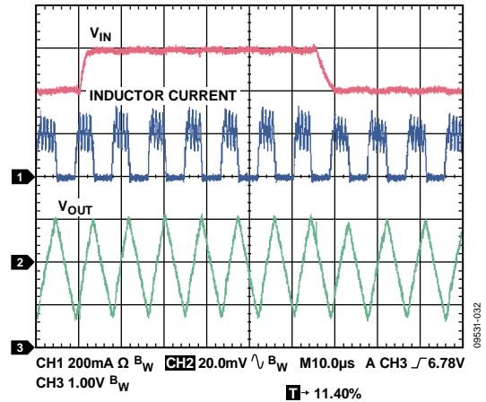
Figure 32. Line Transient, V_{OUT} = 3.3\text{ V} , PSM Mode, 100 mA, V_{IN} = 6\text{ V} to 7 V, 2 \mu\text{s} Rise Time, C_{IN} = 3.3\text{ }\mu\text{F}
