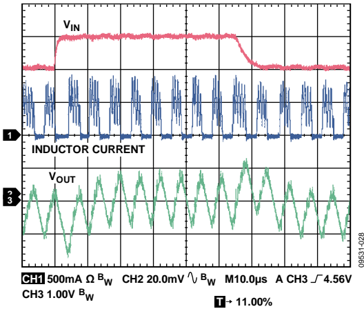
Figure 28. Line Transient, V_{OUT} = 1.8\text{ V} , PSM Mode, 100 mA, V_{IN} = 4\text{ V} to 5 V, 2 \mu\text{s} Rise Time, C_{IN} = 3.3\text{ }\mu\text{F}
