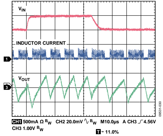
Figure 30. Line Transient, V_{OUT} = 1.2\text{ V} , PSM Mode, 100 mA, V_{IN} = 4\text{ V} to 5 V, 2 \mu\text{s} Rise Time, C_{IN} = 3.3\text{ }\mu\text{F}
