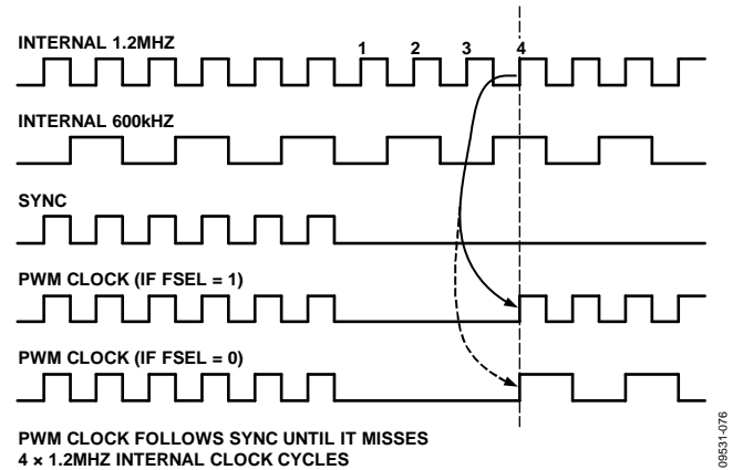
Figure 76. Typical SYNC Timing
