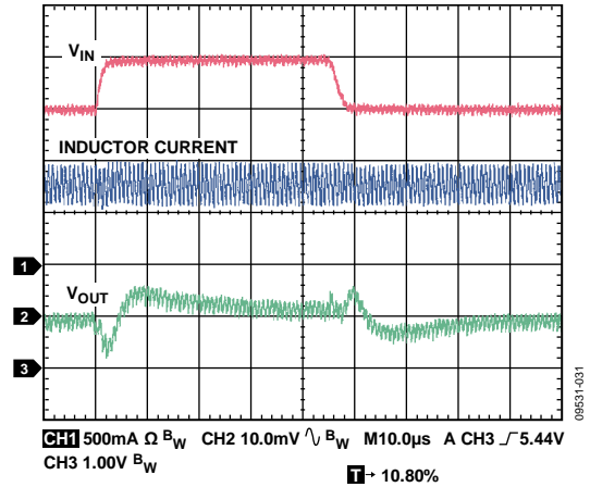
Figure 31. Line Transient, V_{OUT} = 1.2\text{ V} , PWM Mode, 800 mA, V_{IN} = 4\text{ V} to 5 V, 2 \mu\text{s} Rise Time, C_{IN} = 3.3\text{ }\mu\text{F}
