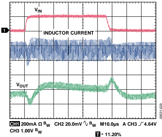
Figure 29. Line Transient, V_{OUT} = 1.8\text{ V} , PWM Mode, 800 mA, V_{IN} = 4\text{ V} to 5 V, 2 \mu\text{s} Rise Time, C_{IN} = 3.3\text{ }\mu\text{F}
