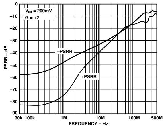
TPC 34. PSRR vs. Frequency
