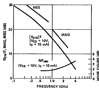
Figure 2. Typical |S_{21}|^2 , MAG, Maximum Stable Gain (MSG), and Noise Figure vs. Frequency for the HXTR-3101 and HXTR-3103.
