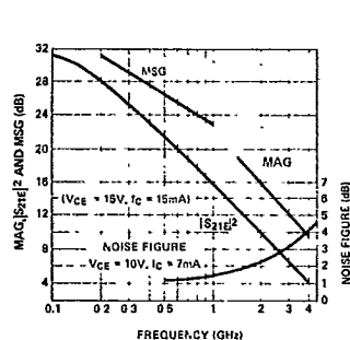
Figure 1. Typical MAG, |S_{21}|^2 , Maximum Stable Gain (MSG), and Noise Figure ( \text{NF}_{\text{MIN}} ) vs. Frequency for the HXTR-3001.
