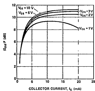
Figure 7. Typical |S_{21}|^2 vs. Collector Current at 1000 MHz for the HSMX-3131.
