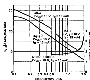
Figure 3. Typical |S_{21}|^2 , MAG, Maximum Stable Gain (MSG), and Noise Figure vs. Frequency for the HSMX-3131.
