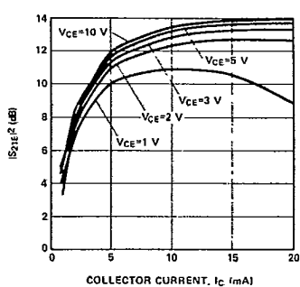
Figure 8. Typical |S_{21}|^2 vs. Collector Current at 1 GHz for the HSMX-3151.
