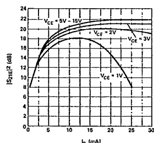
Figure 5. Typical |S_{21}|^2 vs. Collector Current at 500 MHz for the HXTR-3001.
