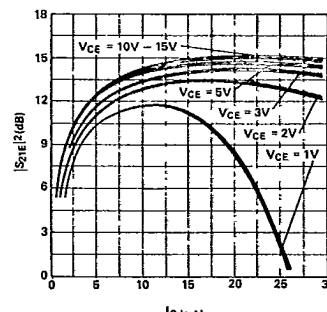
Figure 6. Typical |S_{21}|^2 vs. Collector Current at 1000 MHz for the HXTR-3101 and HXTR-3103.
