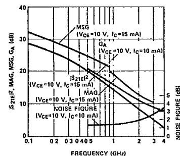
Figure 4. Typical |S_{21}|^2 , MAG, Maximum Stable Gain (MSG), Noise Figure, and G_A vs. Frequency for the HSMX-3151.
