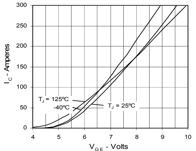
Fig. 6. Input Admittance
