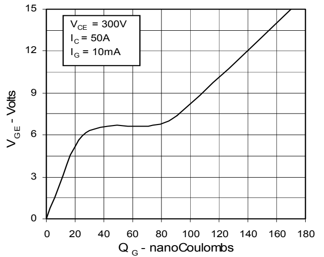
Fig. 14. Gate Charge
