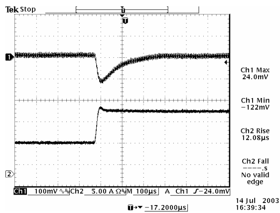
50% to 100% load Transient at V_{in}=5\text{ V} , V_o=3.3\text{ V}
