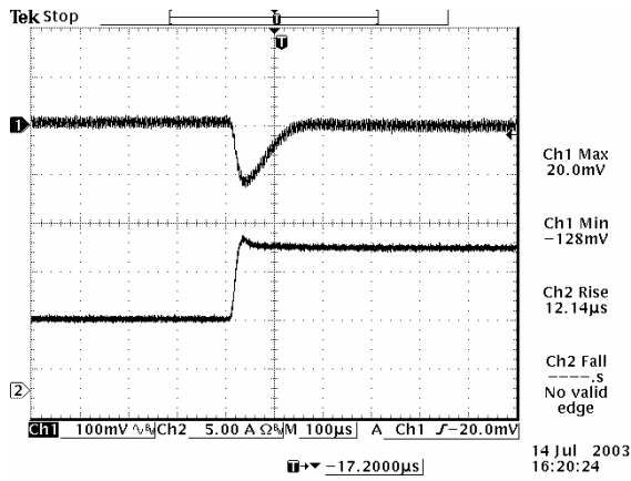
50% to 100% load Transient at V_{in}=5\text{ V} , V_o=1.8\text{ V}
