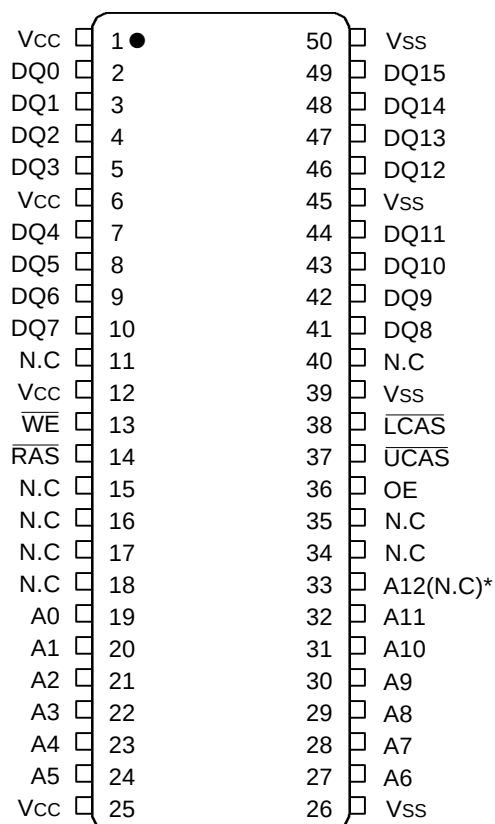
50Pin Plastic TSOP- II (400mil)
