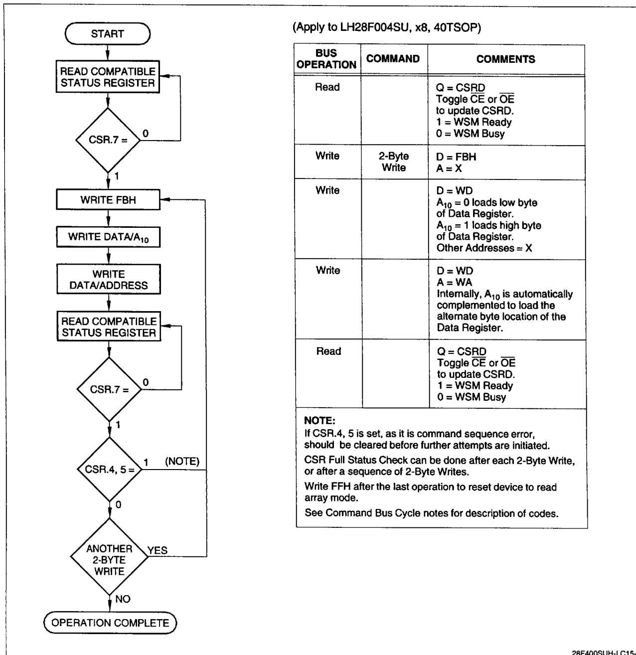
Figure 11. Two-Byte SerialWrites with Compatible Status Registers (40-pin TSOP)
