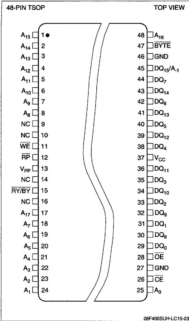
Figure 2. 48-Pin TSOP Configuration
