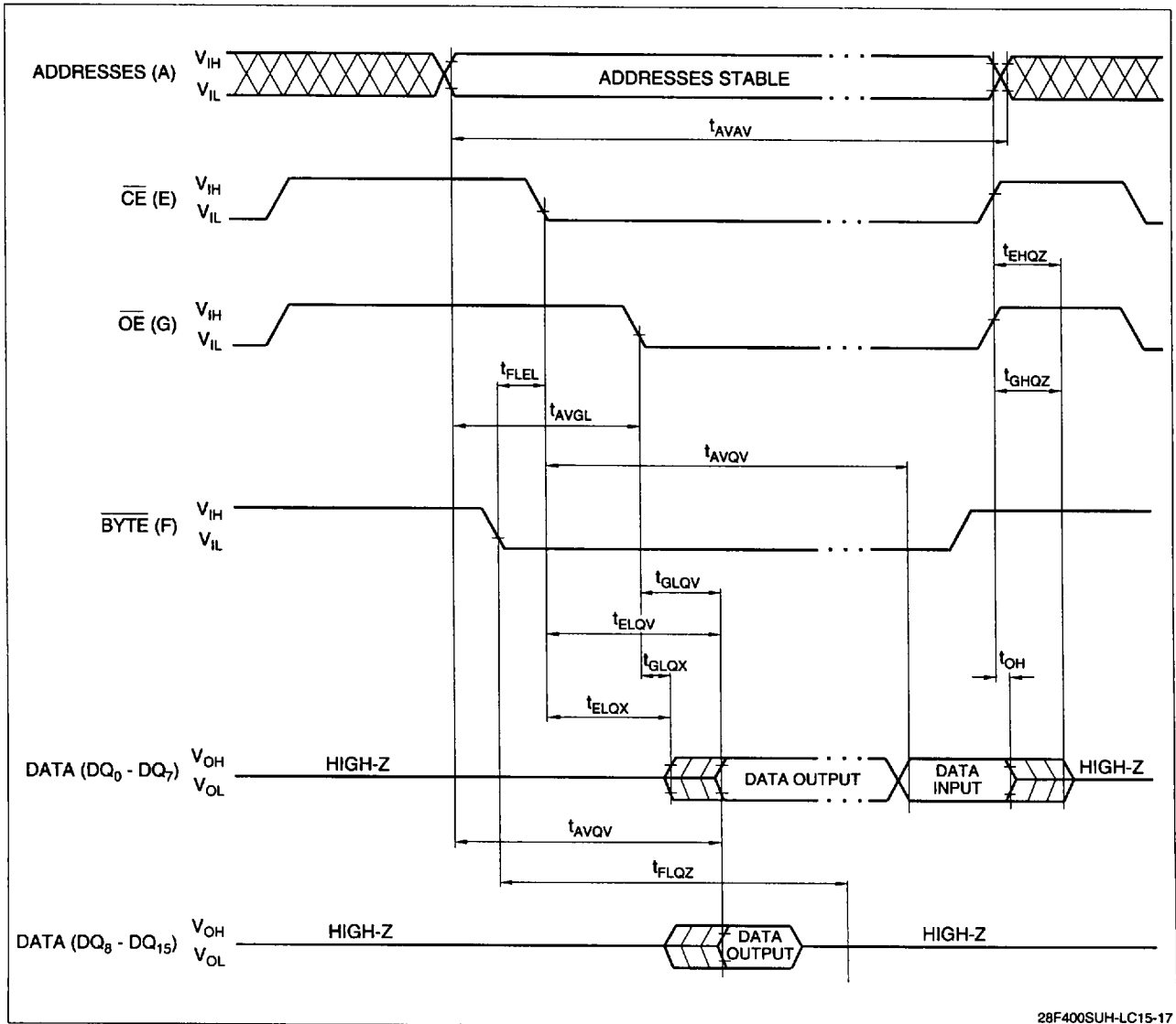
Figure 19. \overline{BYTE} Timing Waveforms
