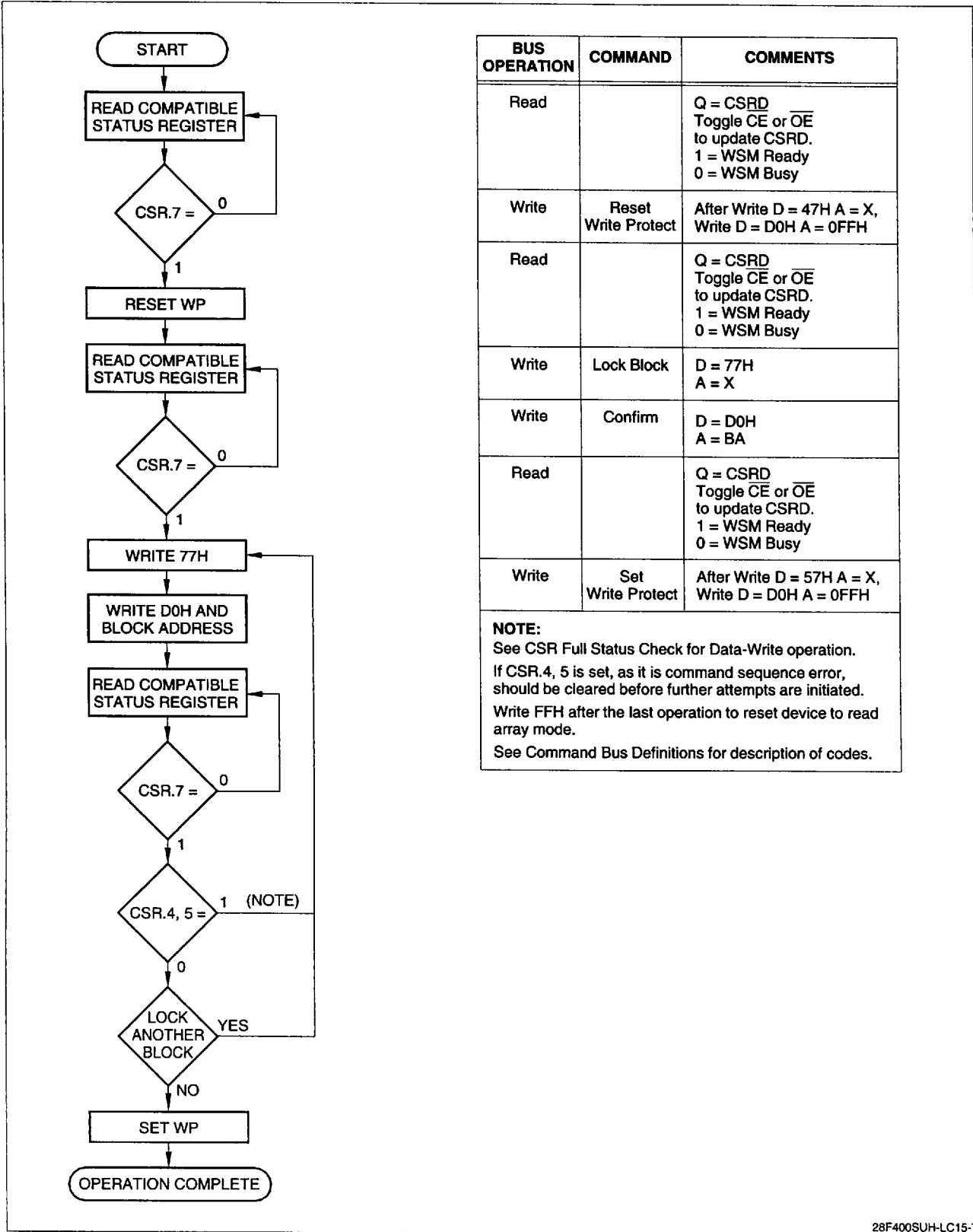
Figure 9. Block Locking Scheme
