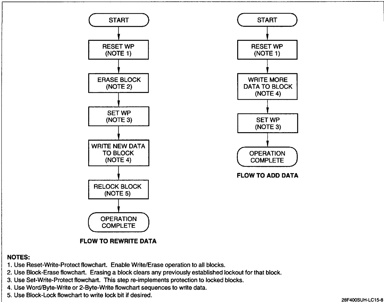
Figure 10. Updating Data in a Locked Block
