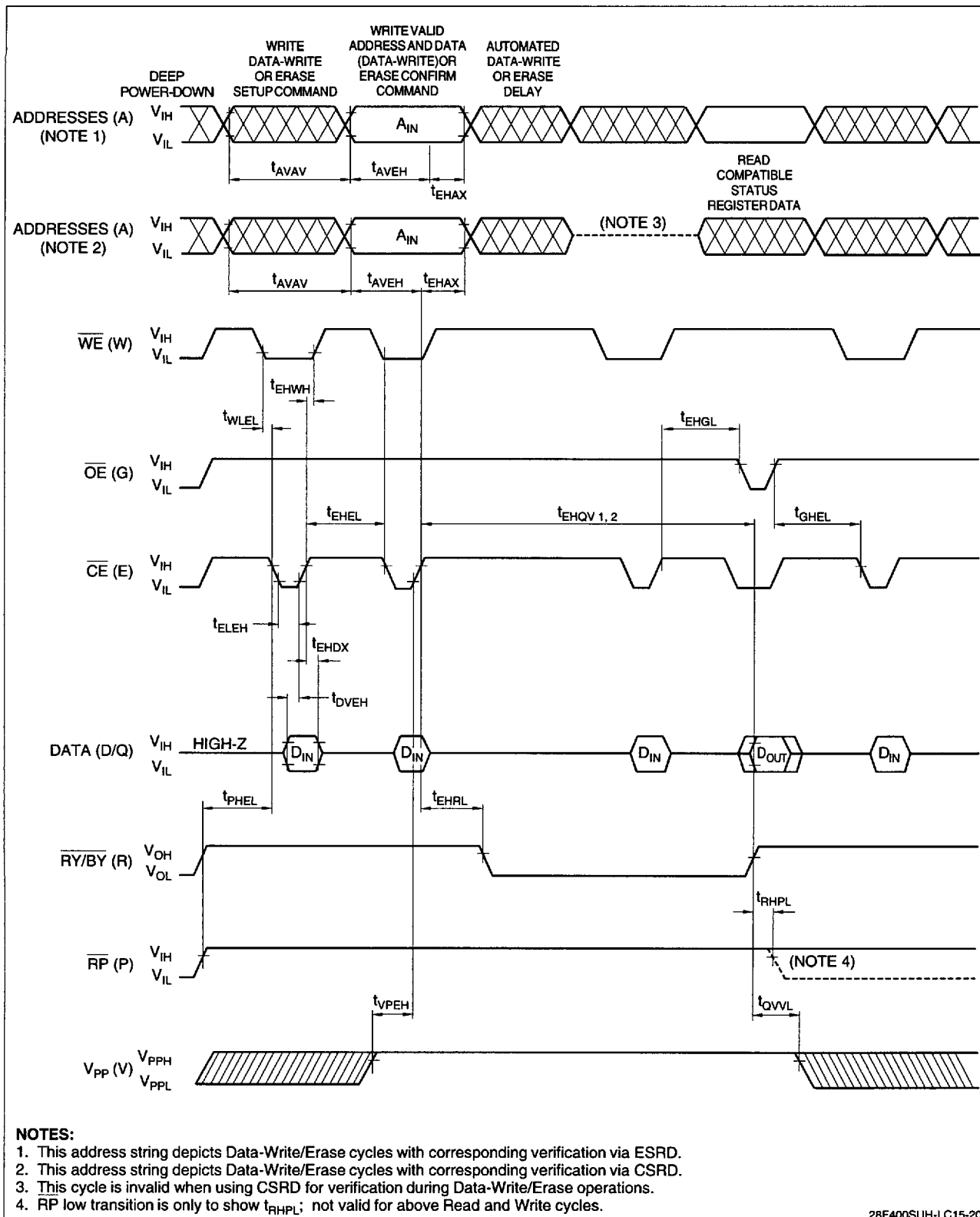
Figure 20. Alternate AC Waveforms for Command Write Operations
