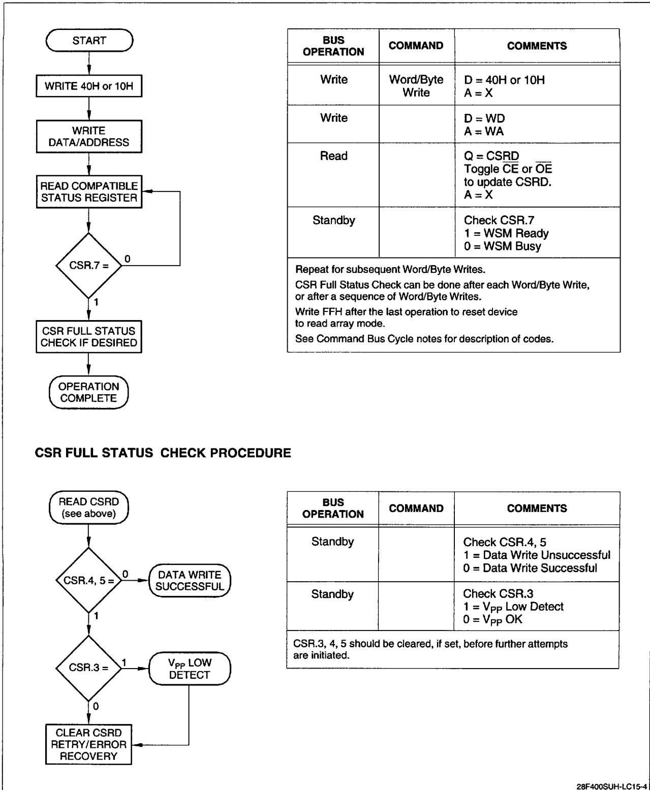
Figure 6. Word/Byte Writes with Compatible Status Register
