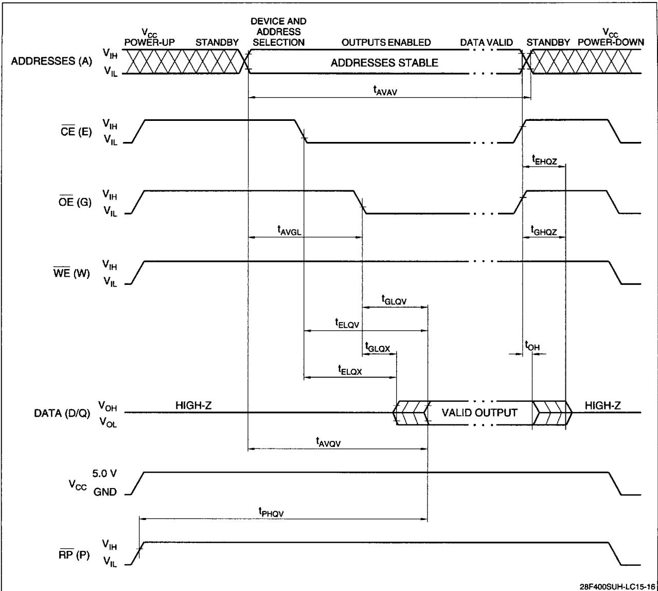
Figure 18. Read Timing Waveforms
