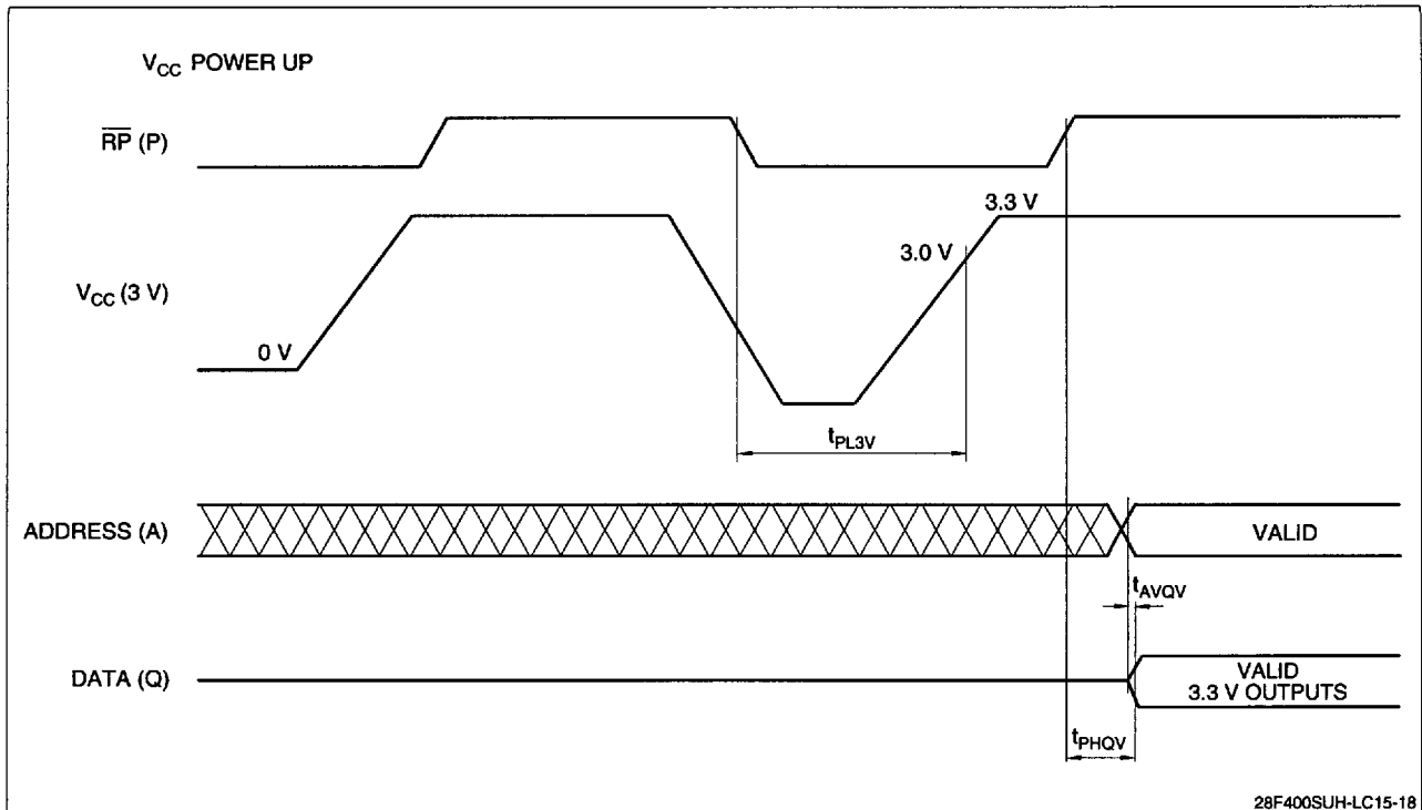
Figure 18. V_{CC} Power-Up and \overline{RP} Reset Waveforms
