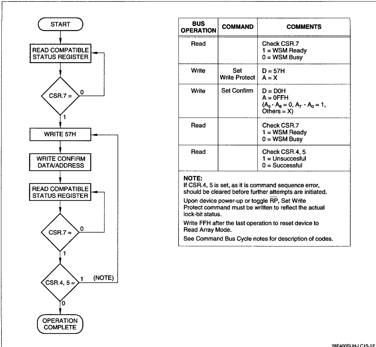
Figure 14. Set Write Protect
