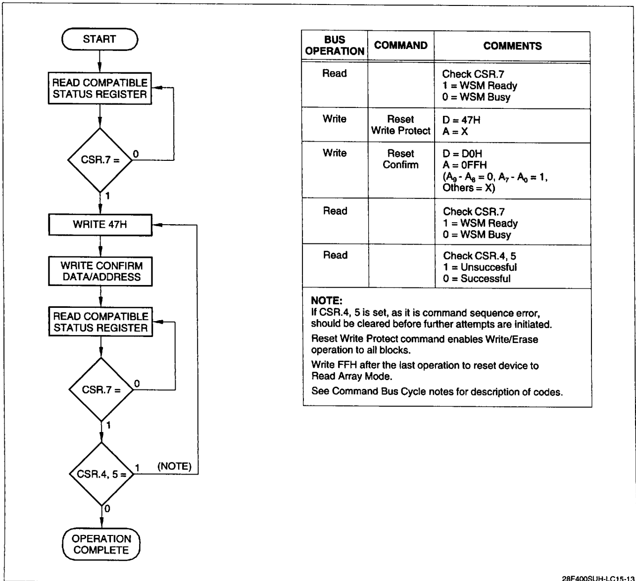
Figure 15. Reset Write Protect
