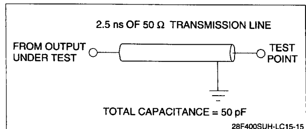
Figure 17. Transient Equivalent Testing Load Circuit ( V_{CC} = 3.3 V)
