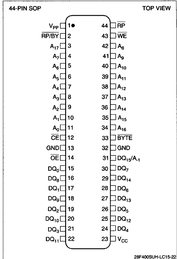
Figure 3. 44-Pin SOP Configuration
