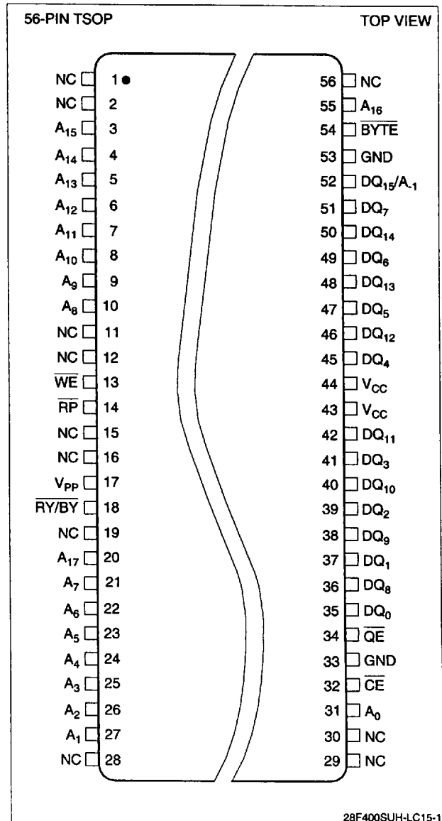
Figure 1. 56-Pin TSOP Configuration
