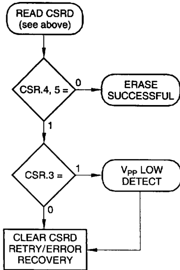
Figure 7. Block Erase with Compatible Status Register
