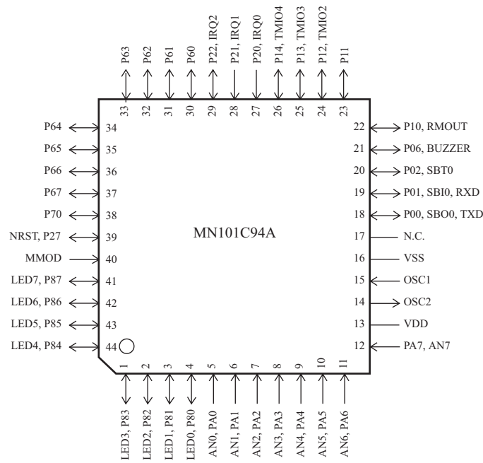
QFP044-P-1010F
