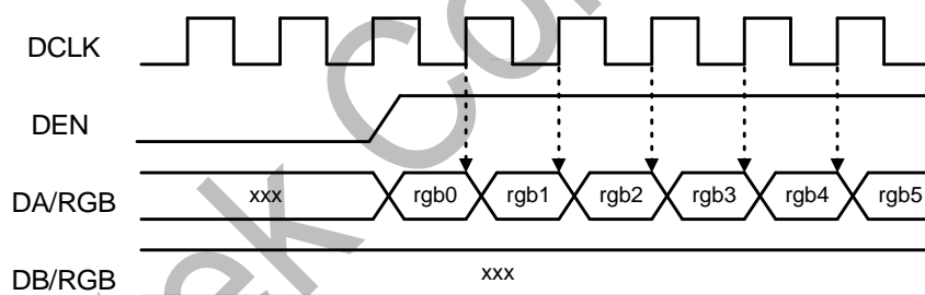
Figure 4 TTL Single Pixel Mode Display Data Timing
