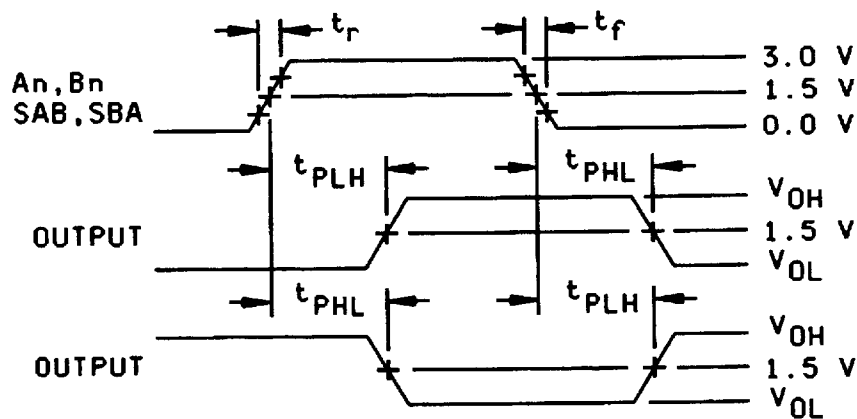
FIGURE 5. Switching waveforms and test circuit
