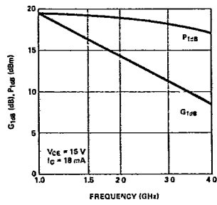
Figure 27. Typical Power Output at 1 dB Compression Gain vs. Frequency, for the HXTR-3675.
