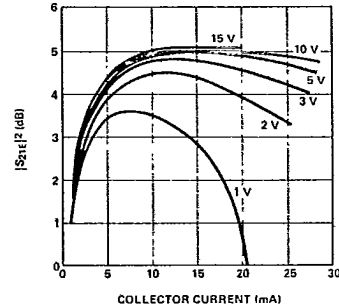
Figure 9. Typical |S_{21}|^2 vs. Collector Current at 4000 MHz, for the HXTR-7111.
