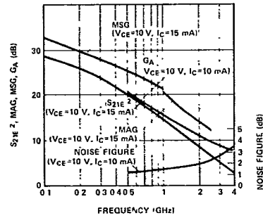
Figure 6. Typical |S_{21}|^2 , MAG, MSG, Noise Figure, and G_A vs. Frequency, for the HSMX-3655.
