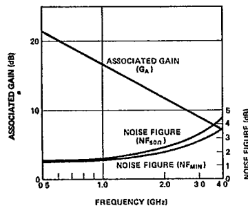
Figure 22. Typical NF_{MIN} and Associated Gain vs. Frequency at V_{CE} = 10\text{ V} , I_C = 10\text{ mA} , for the HXTR-3615.
