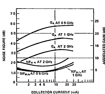
Figure 18. Typical NF_{MIN} and Associated Gain ( G_A ) vs. Collector Current at V_{CE} = 10 V, for the HXTR-3645.
