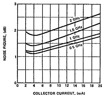
Figure 17. Typical Noise Figure vs. Collector Current, V_{CE} = 10 V, for the HSMX-3635.
