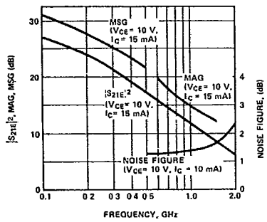
Figure 4. Typical |S_{21}|^2 , MAG, MSG, and Noise Figure vs. Frequency, for the HSMX-3635.
