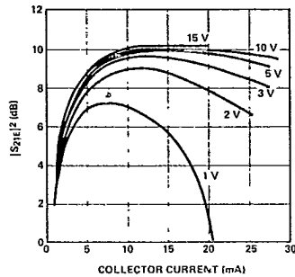
Figure 8. Typical |S_{21}|^2 vs. Collector Current at 2000 GHz, for the HXTR-7011.
