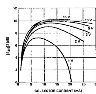
Figure 12. Typical |S_{21}|^2 vs. Current at 2000 MHz, for the HXTR-3645.
