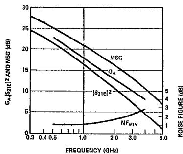
Figure 1. Typical NF MIN , GA, |S 21 | 2 and MSG vs. Frequency at V CE = 10 V, I C = 10 mA for the HXTR-7011.
