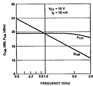
Figure 26. Typical Power Output at 1 dB Compression Gain vs. Frequency, for the HXTR-3645.
