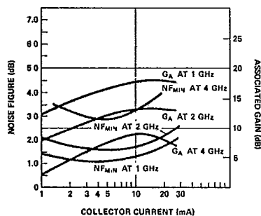
Figure 16. Typical NF_{MIN} and Associated Gain ( G_A ) vs. Collector Current at V_{CE} = 10 V, for the HXTR-7111.
