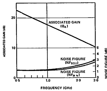
Figure 23. Typical Noise Figure and Associated Gain vs. Frequency at V_{CE} = 10\text{ V} , I_C = 10\text{ mA} , for the HXTR-3645.
