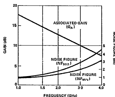
Figure 21. Typical Noise Figure and Associated Gain vs. Frequency at V_{CE} = 10 V, I_C = 10 mA, for the HXTR-7111.
