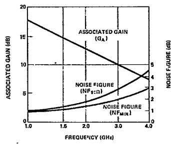
Figure 24. Typical Noise Figure and Associated Gain vs. Frequency at V_{CE} = 10\text{ V} , I_C = 10\text{ mA} , for the HXTR-3675.
