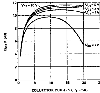
Figure 11. Typical |S_{21}|^2 vs. Collector Current at 1000 MHz, for the HSMX-3635.
