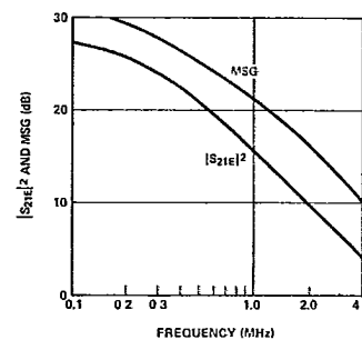
Figure 3. Typical |S 21 | 2 and Maximum Stable Gain (MSG) vs. Frequency at V CE = 10 V and I C = 10 mA, for the HXTR-7111.
