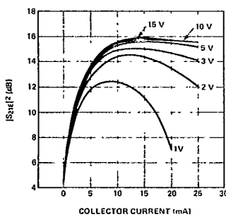
Figure 10. Typical |S_{21}|^2 vs. Collector Current at 1000 MHz, for the HXTR-3615.
