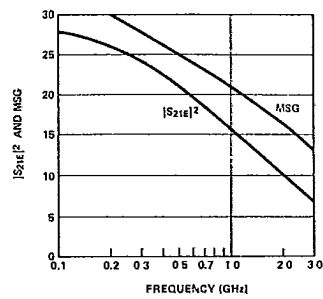
Figure 5. Typical |S_{21}|^2 and Maximum Stable Gain (MSG) vs. Frequency at V_{CE} = 10 V and I_C = 10 mA, for the HXTR-3645.
