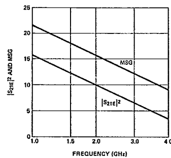
Figure 2. Typical |S 21 | 2 and Maximum Stable Gain (MSG) vs. Frequency at V CE = 10 V and I C = 10 mA, for the HXTR-7111.
