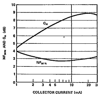
Figure 15. Typical NF_{MIN} and Associated Gain vs. I_C at 4 GHz for V_{CE} = 10 V, for the HXTR-7011.
