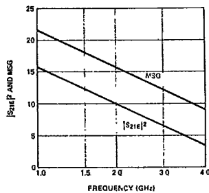
Figure 7. Typical |S_{21}|^2 and Maximum Stable Gain (MSG) vs. Frequency at V_{CE} = 10 V and I_C = 10 mA, for the HXTR-3675.
