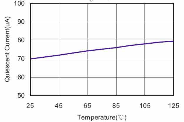
8. Quiescent Current vs Temperature
