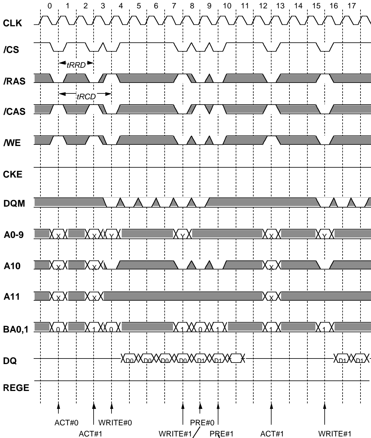
Write Interrupted by Precharge BL=4, Latch mode(REGE="H")
