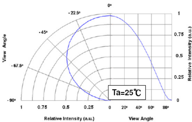
Radiation Pattern
