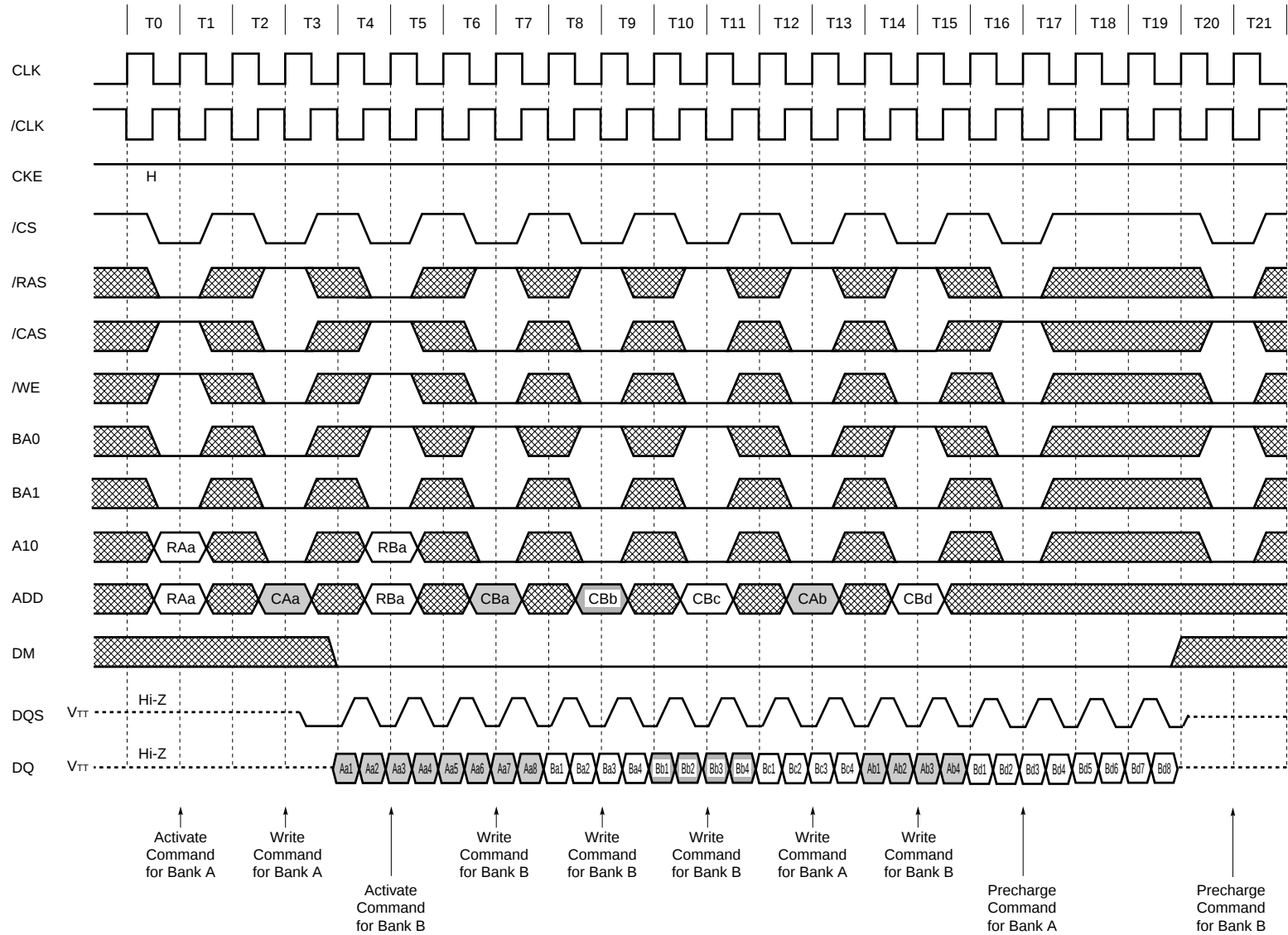
Interleaved Column Write Cycle (1/2) (Burst Length = 8, /CAS Latency = 2)
