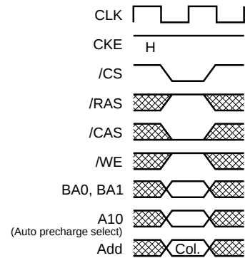
Fig.5 Read command
