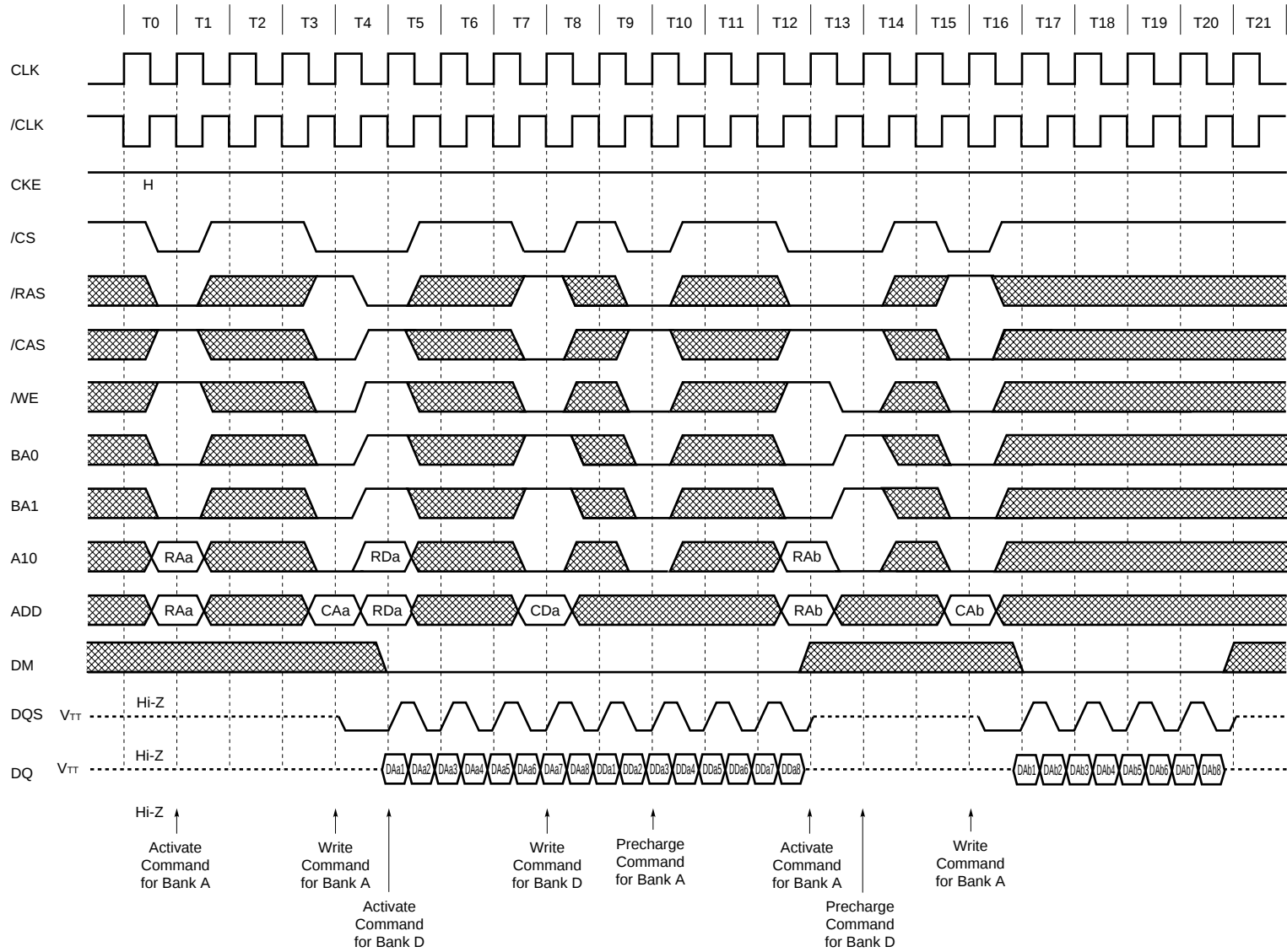
Random Row Write (Ping-Pong Banks) (2/2) (Burst Length = 8, /CAS Latency = 2.5)
