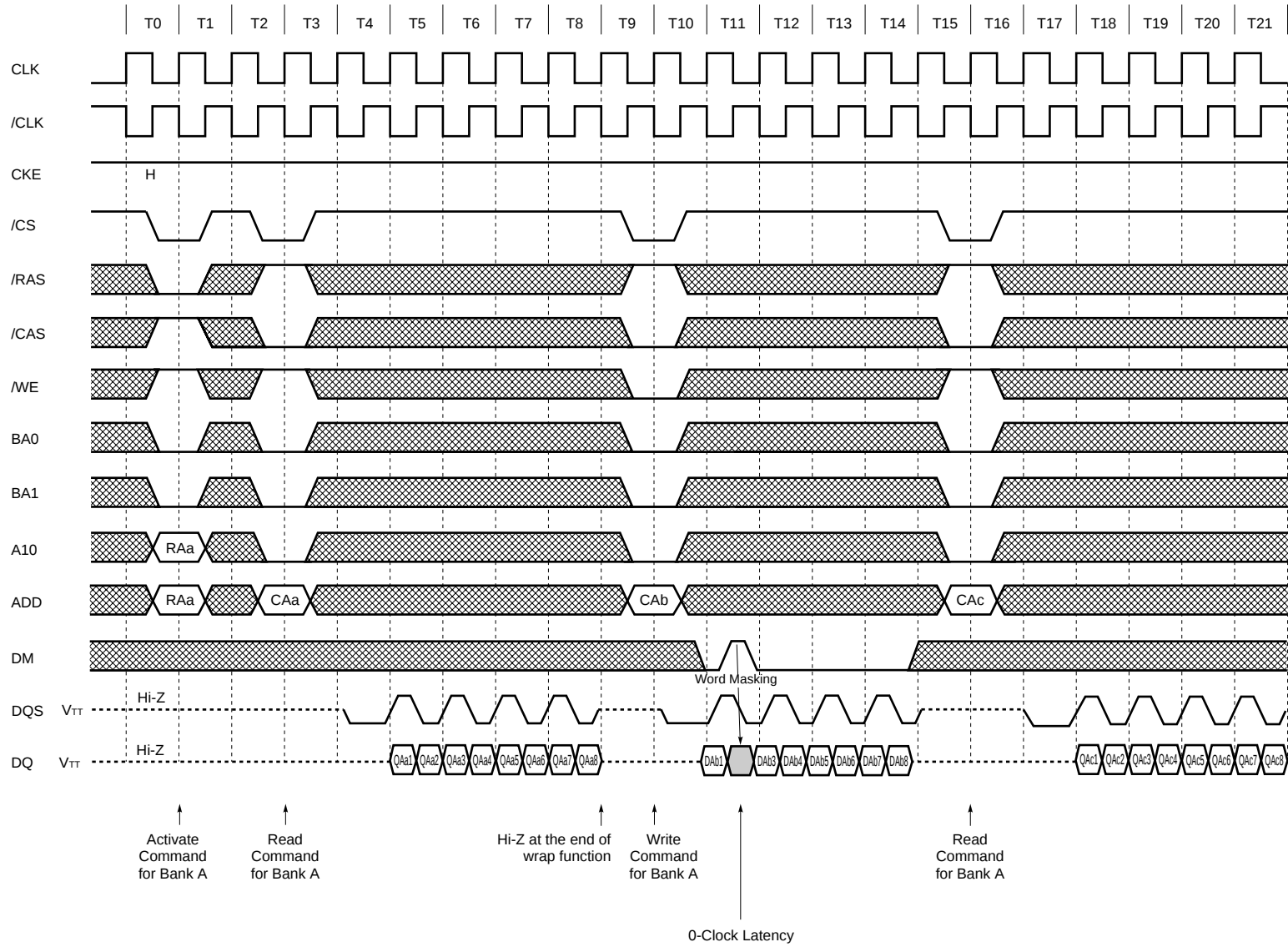
Read and Write (1/2) (Burst Length = 8, /CAS Latency = 2)
