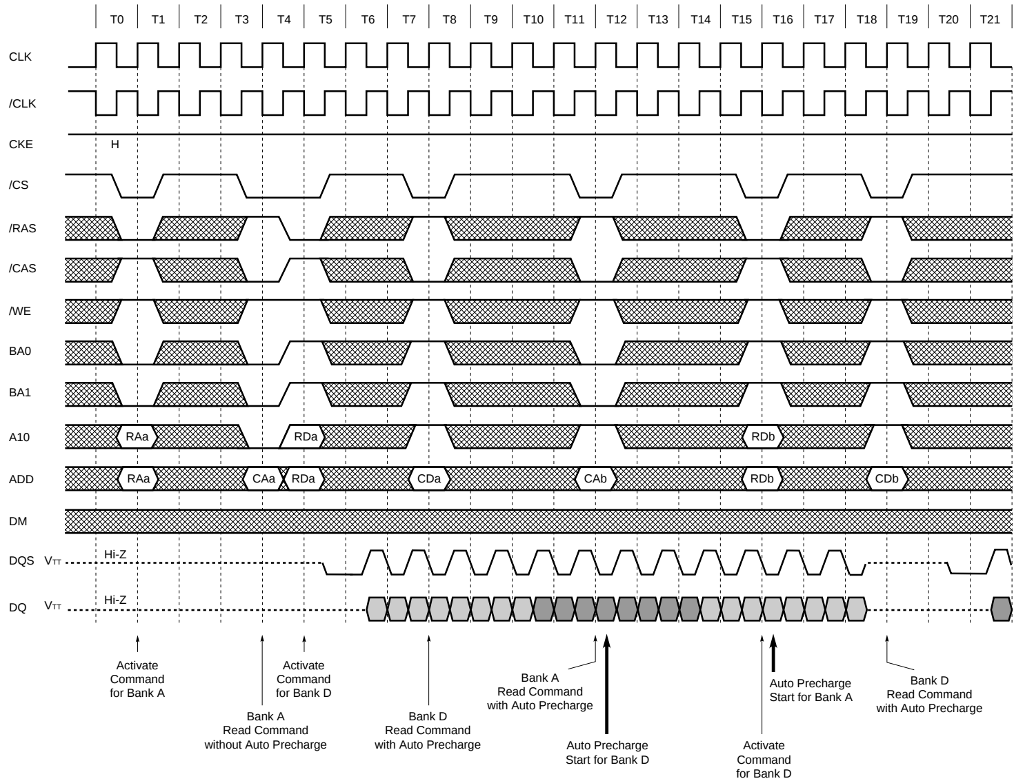
Auto Precharge after Read Burst (2/2) (Burst Length = 8, /CAS Latency = 2.5)
