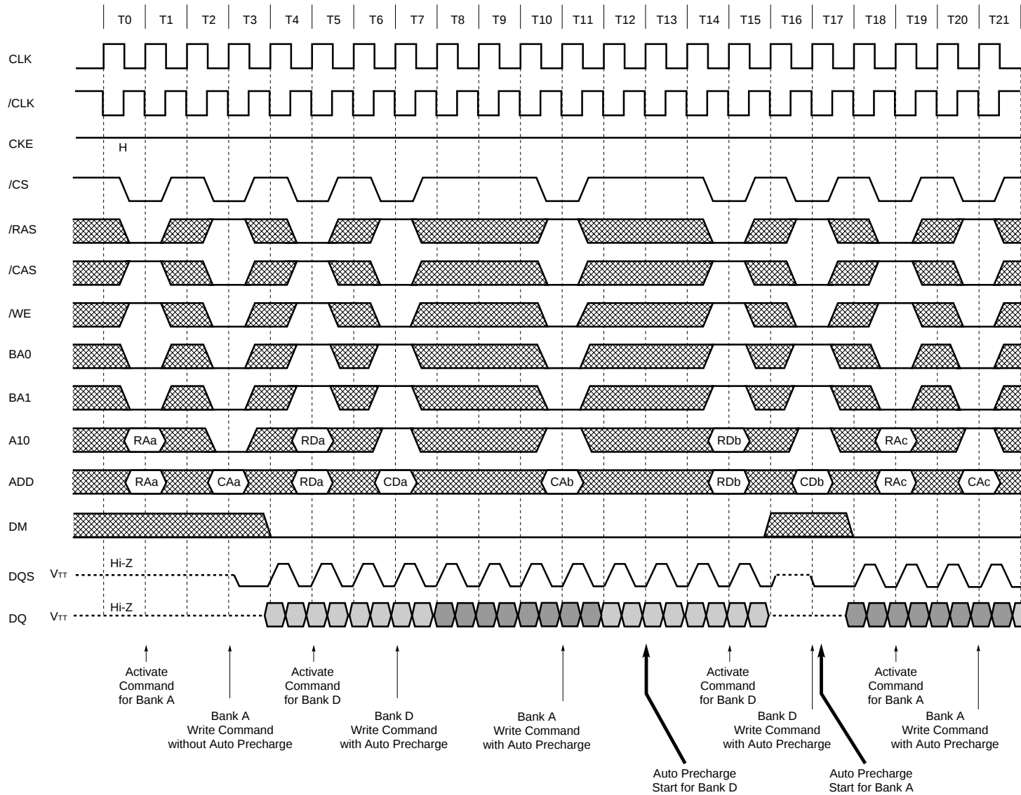
Auto Precharge after Write Burst (1/2) (Burst Length = 8, /CAS Latency = 2)
