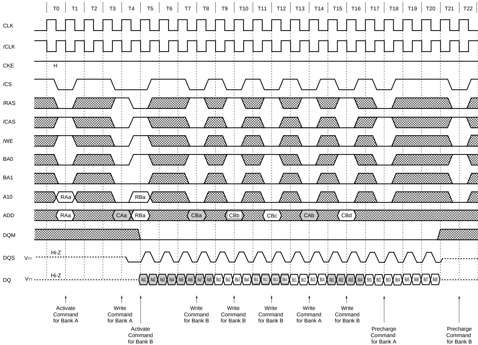
Interleaved Column Write Cycle (2/2) (Burst Length = 8, /CAS Latency = 2.5)
