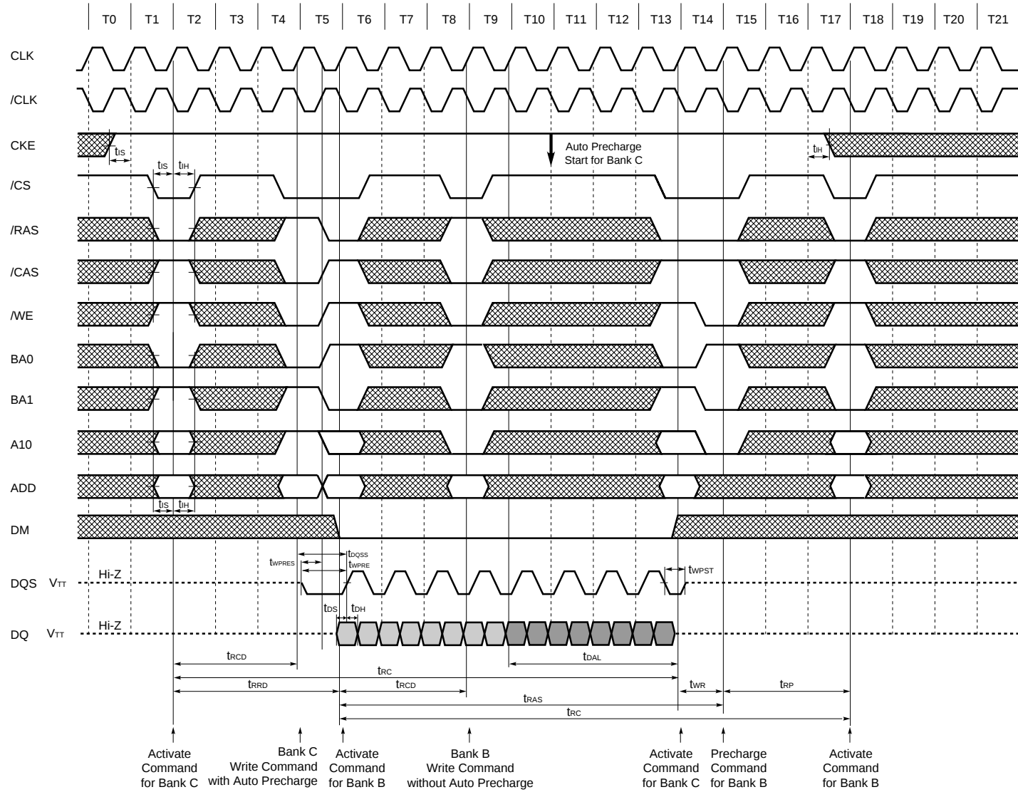
AC Parameters for Write Timing (Burst Length = 8, /CAS Latency = 2.5)
