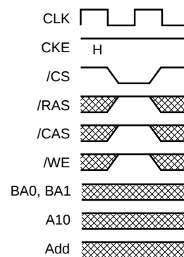
Fig.10 No operation
