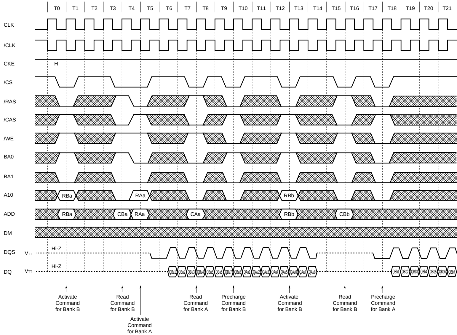
Random Row Read (Ping-Pong Banks) (2/2) (Burst Length = 8, /CAS Latency = 2.5)
