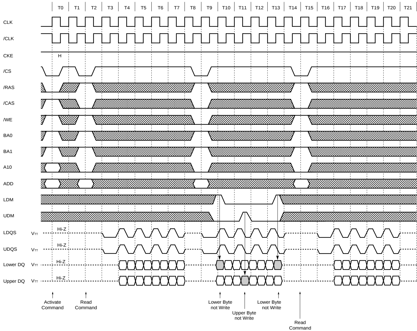
Byte Write Operation (Burst Length = 8, /CAS Latency = 2)
