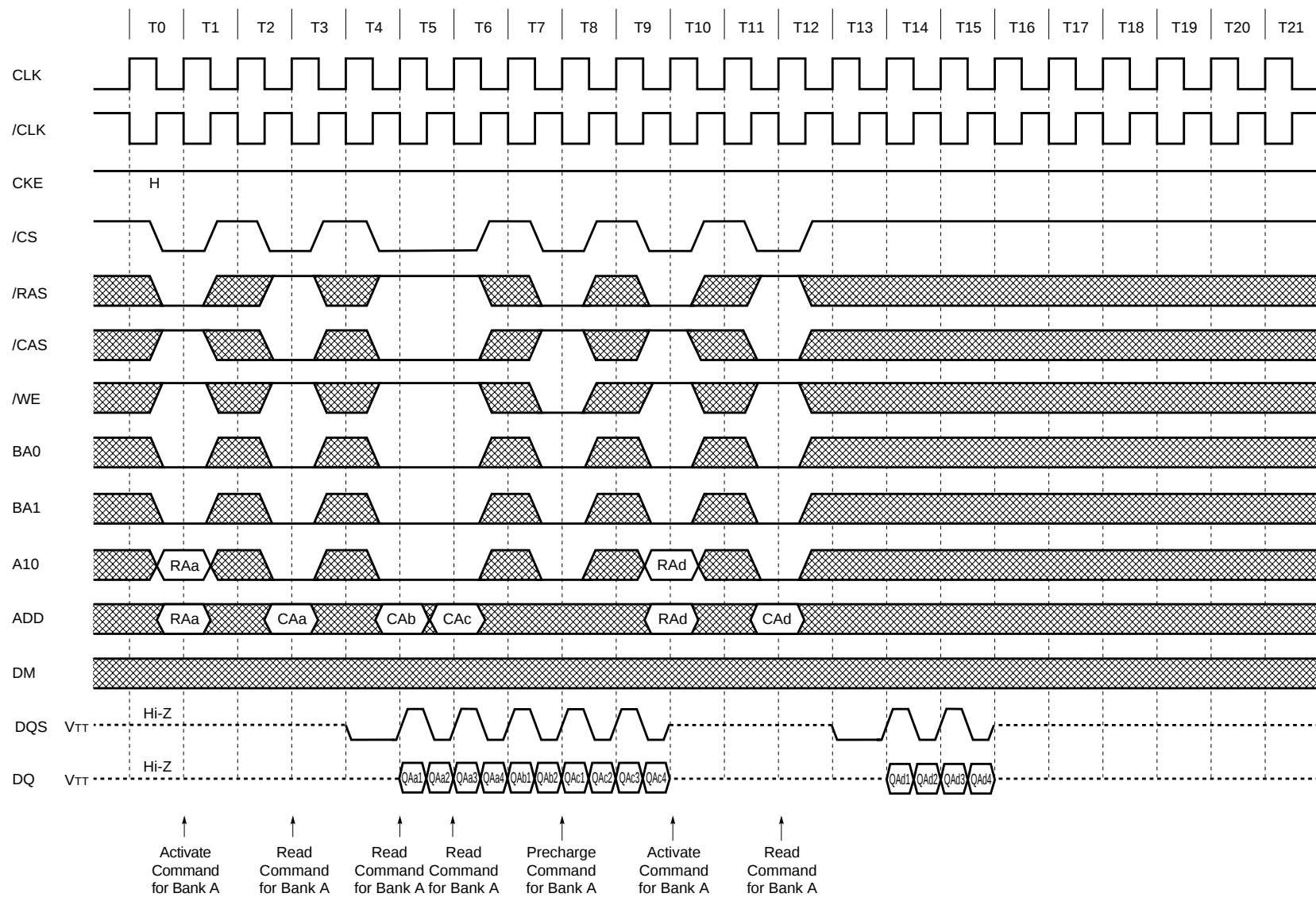
Random Column Read (Page with Same Bank) (1/2) (Burst Length = 4, /CAS Latency = 2)
