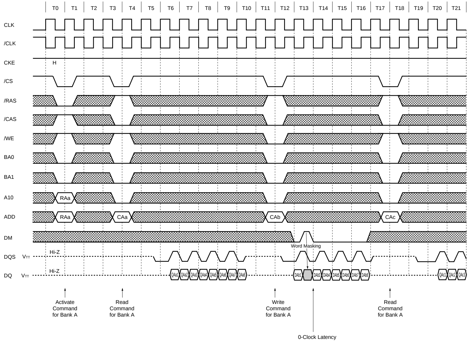
Read and Write (2/2) (Burst Length = 8, /CAS Latency = 2.5)
