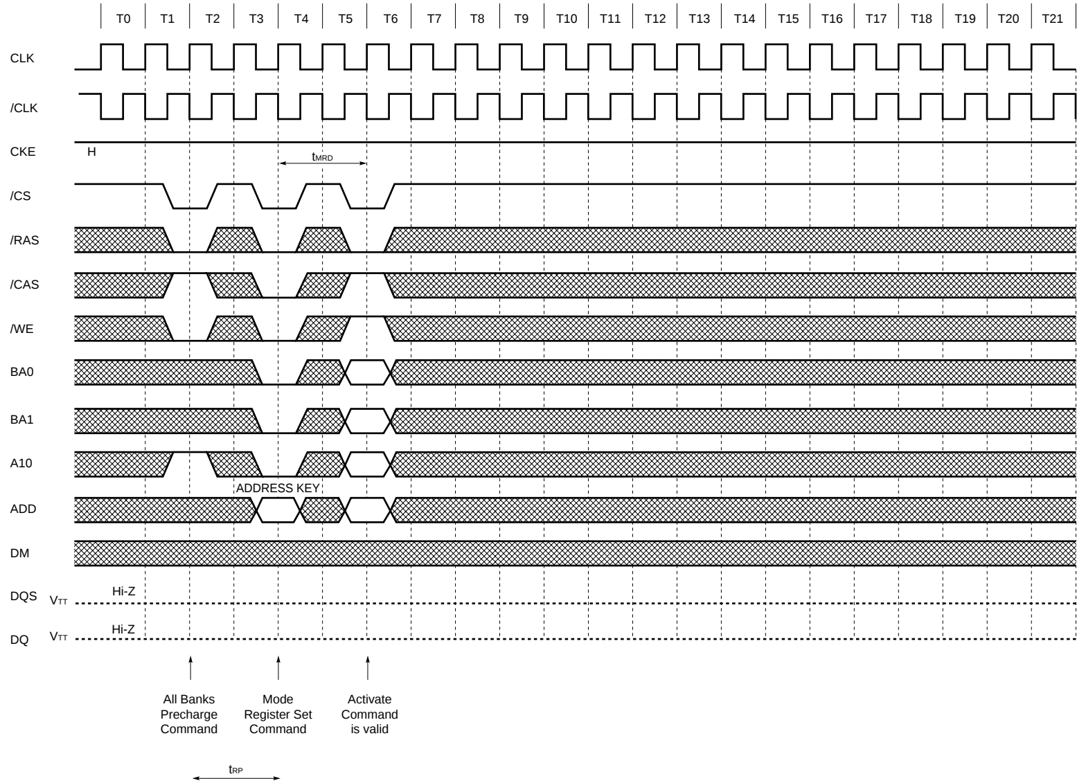
Mode Register Set (Burst Length = 4, /CAS Latency = 2)
