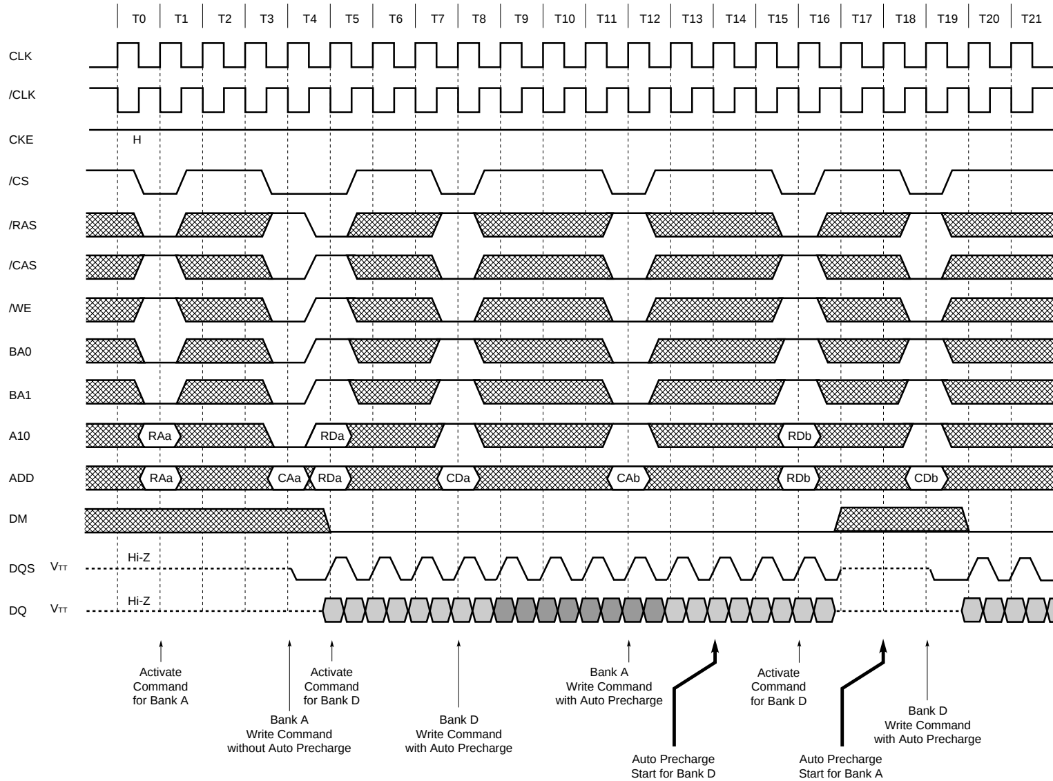
Auto Precharge after Write Burst (2/2) (Burst Length = 8, /CAS Latency = 2.5)
