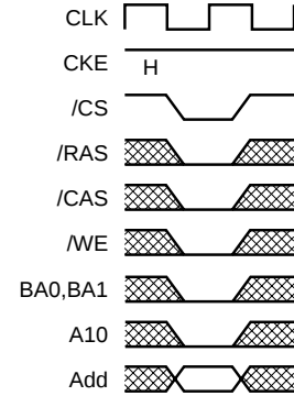
Fig.2 Mode register set command
