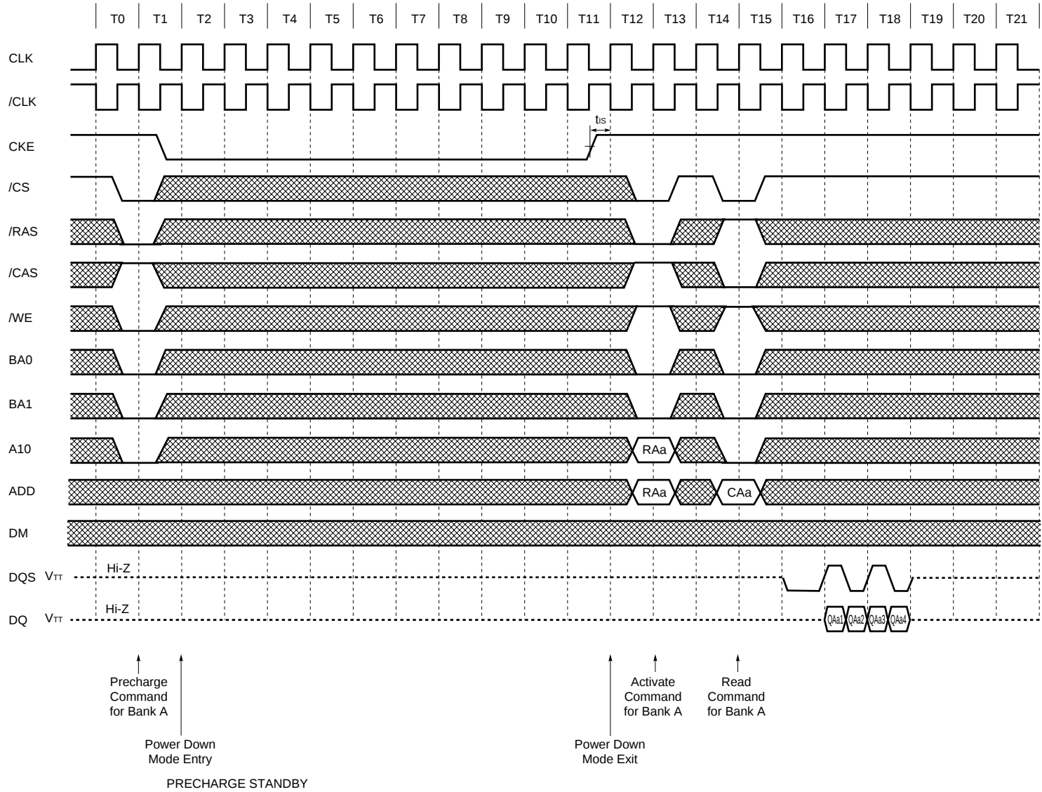
Power Down Mode (Burst Length = 4, /CAS Latency = 2)
