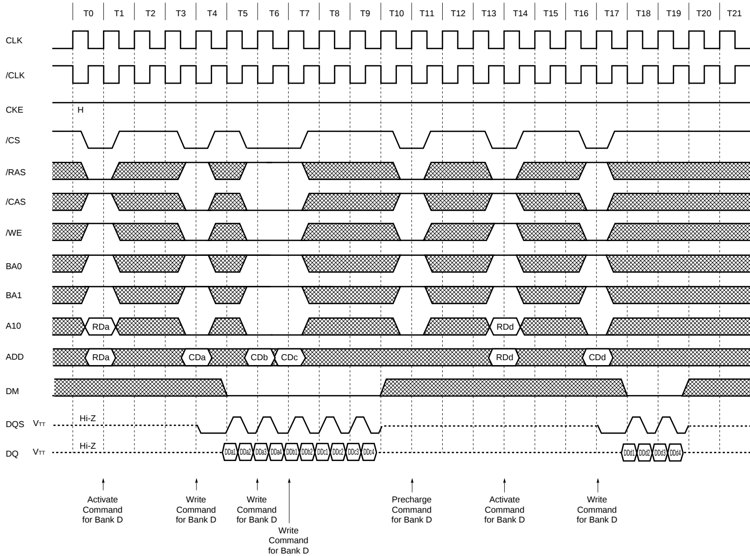
Random Column Write (Page with Same Bank) (2/2) (Burst Length = 4, /CAS Latency = 2.5)
