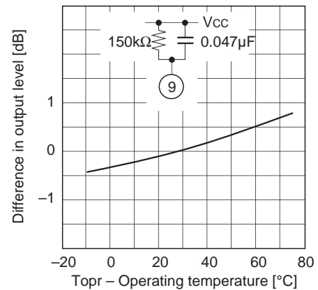
AGC output level vs. Operating temperature
