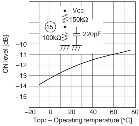
Dropout detection ON level vs. Operating temperature
